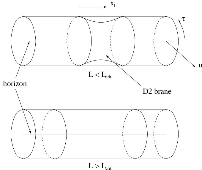
Figure 2: For L > L_{\text{crit}} , there is no volume-minimizing D2 brane configuration connection the m - \bar{m} pair
