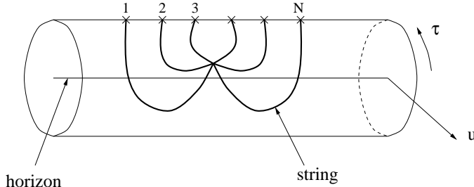
Figure 9: Baryon is constructed as N strings joining together at a point in the bulk.
