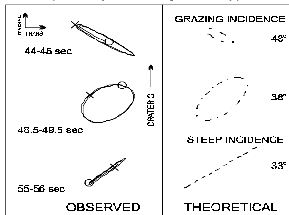
Figure 4. Observed and theoretical particle motions in the horizontal plane. The left column shows a 12 s sequence (0.5-3 Hz bandpass) taken from the second tremor episode ("B") in figure 3. An "x" marks the beginning and an "o" the end of each one-second trace. The particle motion azimuth abruptly rotates clockwise 105°. The right column shows theoretical particle motions on a horizontal free surface due to a shear wave (polarization angle e = 20^\circ , Poisson's ratio =
