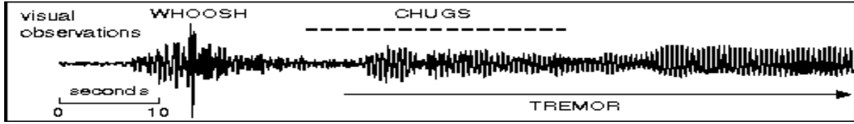
Figure 2. An example seismogram (radial component) of a small eruption (whoosh) followed by rhythmic degassing (chugs). Visual and audio observations show this eruption ejecting ash to ~500 m above the crater and the following chugs were audible at 2.8 km for ~25 s. Harmonic tremor begins during the chugs and continues for several minutes.
