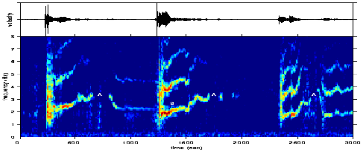
Figure 3. Velocity seismogram and spectrogram (radial component), beginning at 01:05 UT, April 25, 1994, showing three small eruptions. The beginning of the second event is shown in detail in figure 2. The spectra of the volcanic tremor are dominated by narrow peaks spaced regularly in frequency, each of which changes frequency systematically with time. The tremor stops abruptly when the frequency of the first peak reaches ~3.2 Hz (see point "A"). The spectrogram is constructed by stacking 10 s FFT spectra with 50% overlap. Scale bar (right) shows arbitrary units.
