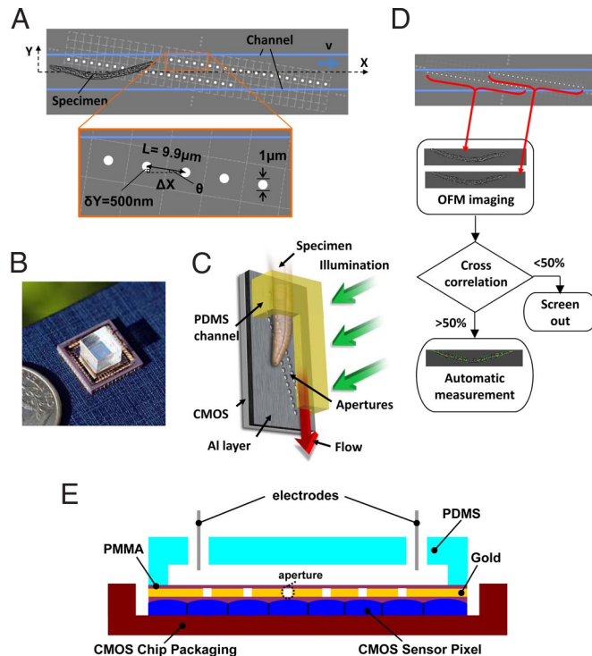
Fig. 2. OFM prototype. (A) schematic of the device (top view). The OFM apertures (white circles) are defined on the Al (gray) coated 2D CMOS image sensor (light gray dashed grid) and span across the whole microfluidic channel (blue lines). (B) The actual device compared with a U.S. quarter. (C) Upright operation mode. (D) Flow diagram of the OFM operation. Two OFM images of the same C. elegans are acquired by the two OFM arrays, respectively (red arrows). If the image correlation is <50%, the image pair is rejected. Otherwise, the area and the length of the worms are measured automatically by evaluating the contour (green dashed line) and the midline (yellow dashed line). (E) Cross-section of the fabrication of an electrokinetically driven OFM device.
