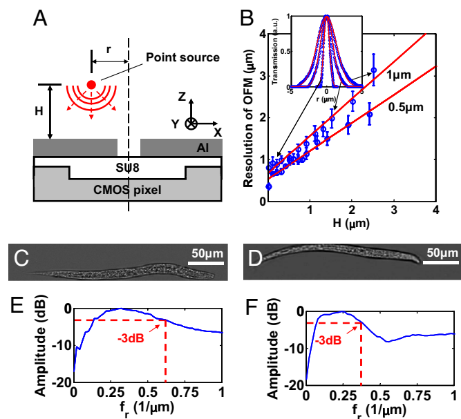
Fig. 6. Resolution of the OFM prototype. (A) Schematic of the PSF measurement. (B) Resolution of the prototype at various heights H above a 0.5- and a 1- \mu\text{m} -diameter aperture under Sparrow's criterion. (Inset) Representative OFM PSF plots at H = 0.1, 1.5, and 2.5 \mu\text{m} for the 1- \mu\text{m} -diameter aperture. (C and D) OFM images of wild-type C. elegans L1 larvae in a 15- and 25- \mu\text{m} -tall microfluidic channels, respectively. (E and F) Radial frequency spectra of OFM images in C and D, respectively. The -3\text{dB} bandwidths (dashed red lines) are at 0.62 and 0.38 \mu\text{m}^{-1} , respectively.
