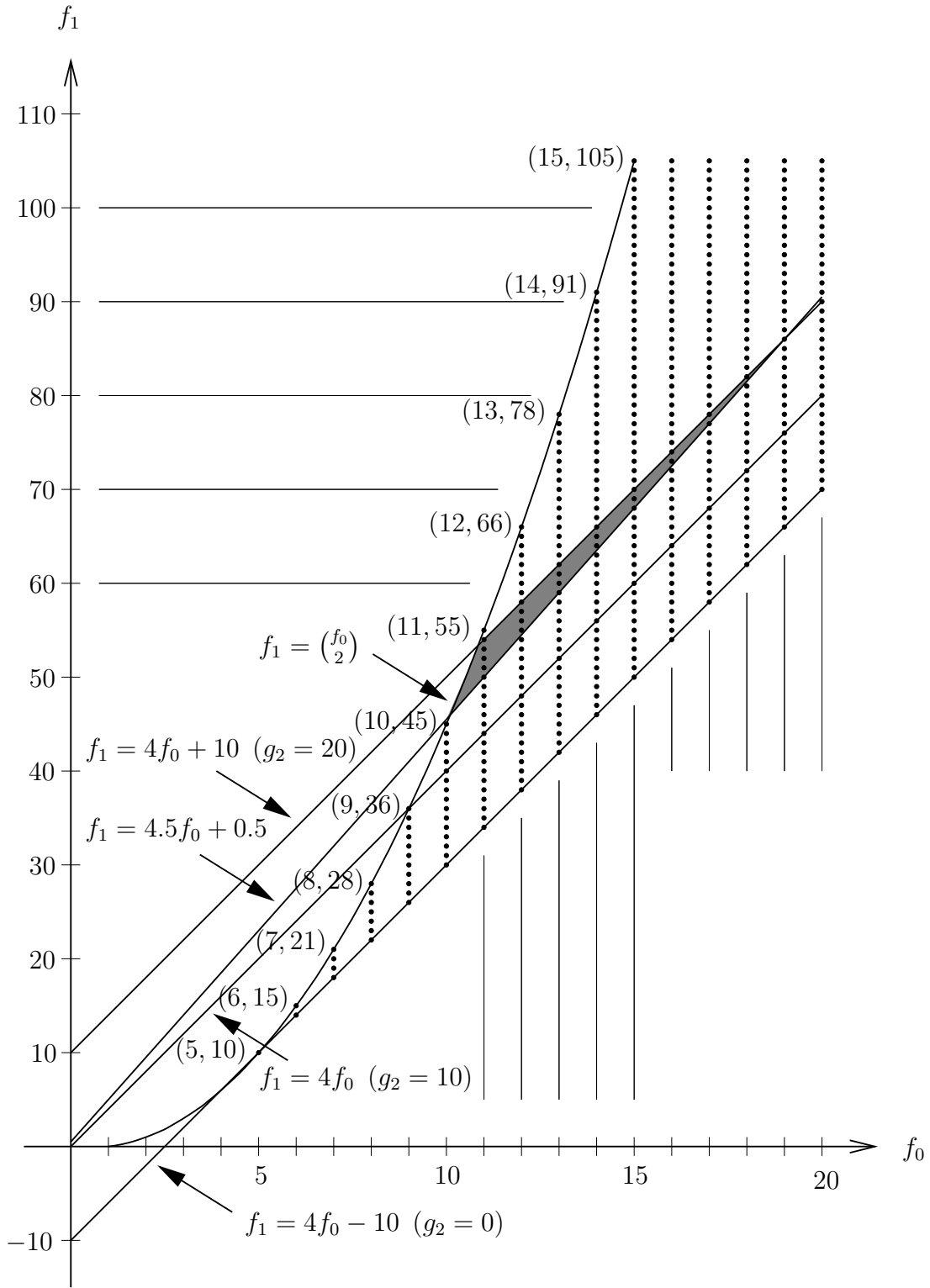
Figure 2: Range (in grey) for g_2 -irreducible triangulations of 3-manifolds with g_2 \leq 20 . The range is bounded by the inequalities f_1 > \frac{9}{2}f_0 + \frac{1}{2} , f_1 - 4f_0 + 10 \leq 20 , and f_1 \leq \binom{f_0}{2} .
