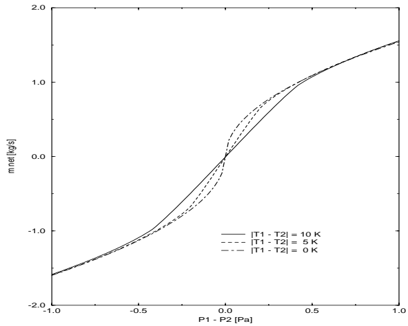
Figure 3 Net mass flow rate \dot{m}_{net} ( \text{kg/s} ) vs pressure difference P_1 - P_2 ( \text{Pa} ) as a function of absolute temperature difference |T_1(z_0) - T_2(z_0)| ( \text{K} )
