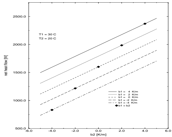
Figure 4 Net heat flow \Phi_{net} ( \text{W} ) vs vertical temperature gradient b_2 ( \text{K/m} ) for zone 2 as a function of gradient b_1 ( \text{K/m} ) for zone 1; \Delta P(z_0) = 0 ( \text{Pa} )
