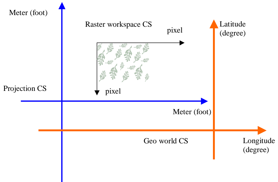
Figure 12: the relationship of the three coordinate systems
