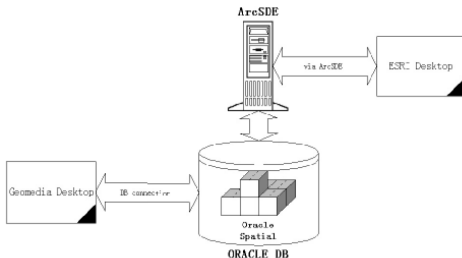
Figure 10: Vector Data sharing for GeoMedia
