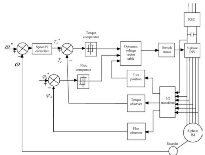
Fig. 15 Block diagram of hysteresis-based DTC for a five-phase induction motor drive
