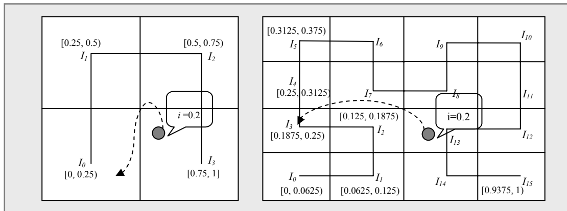
Figure 2. Level 1 and Level 2 Hilbert Curve [22].
