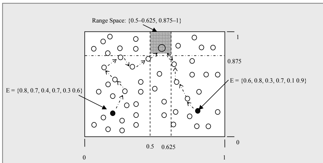
Figure 5. Multidimensional Range Query Mechanism (MDAs) [35].
