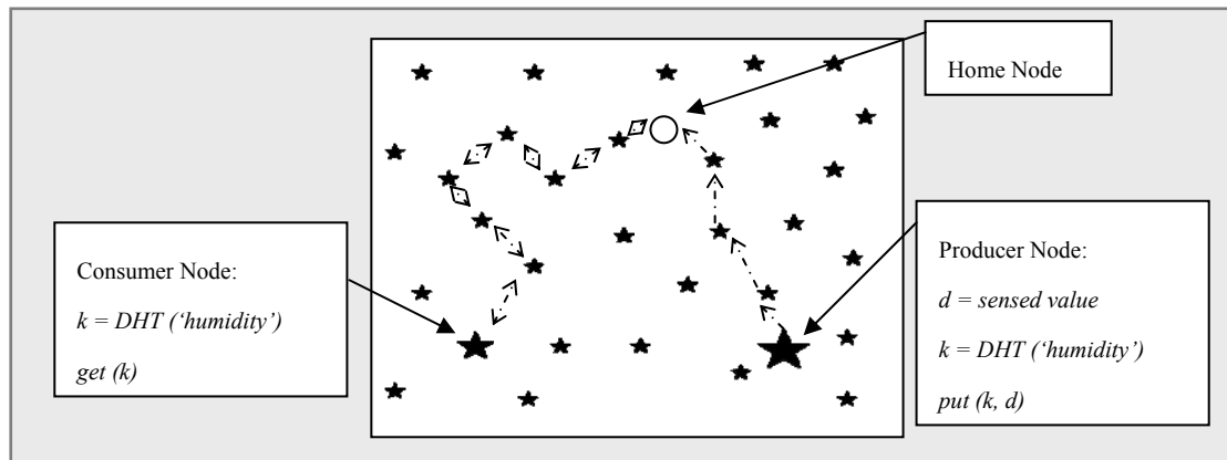
Figure 1. Geographic Hash Table [1].
