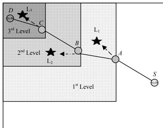
Figure 4. Region Oriented Routing [33].
