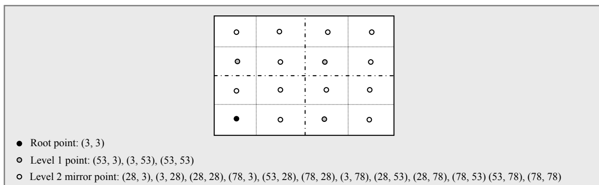
Figure 6. Structured Replication [1].
