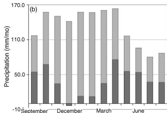
Fig. 7. (a) Mean monthly distribution of excess and deficits for the series 1931–1960 (dark gray) and 1961–1990 (light gray); (b) mean monthly distribution of precipitation into evapotranspiration (light gray) and excess-deficits (dark gray) for the Ibera system.
