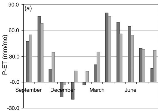
Fig. 7. (a) Mean monthly distribution of excess and deficits for the series 1931–1960 (dark gray) and 1961–1990 (light gray); (b) mean monthly distribution of precipitation into evapotranspiration (light gray) and excess-deficits (dark gray) for the Ibera system.
