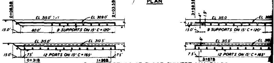
BAFFLE DETAILS AT FLOOR CULVERT MANIFOLDS
