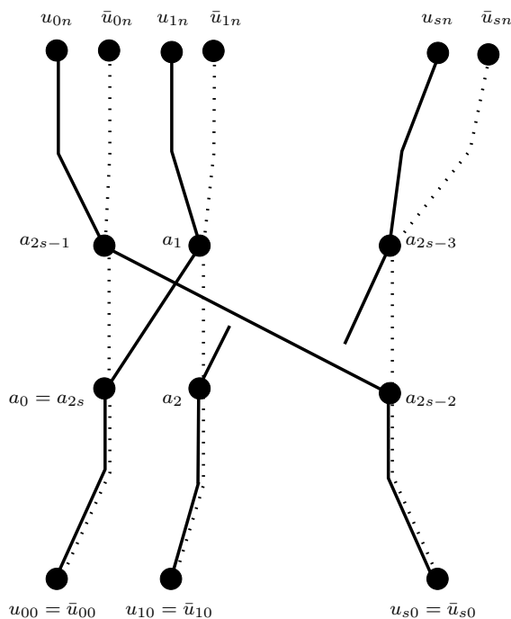
FIGURE 1. A binomial in the Gröbner basis of the ascending model
