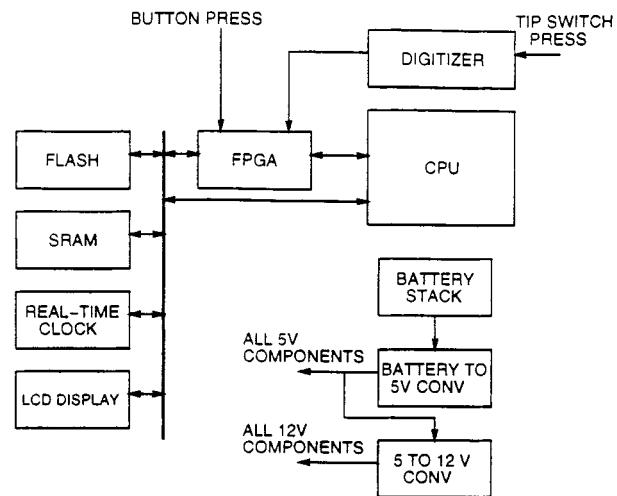
Fig. 3. PaperClip hardware diagram.
