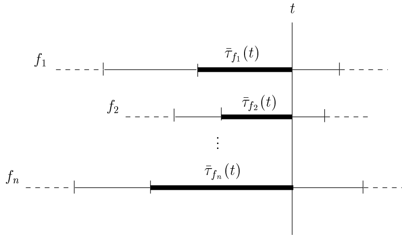
Figure 3: Definition of \bar{\tau}_f .
