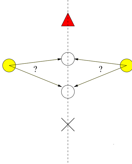
Figure 7: More than 1 position on the axis.
