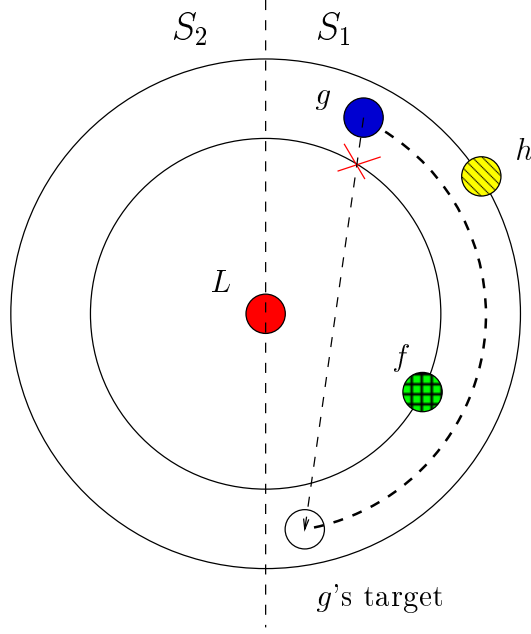
Figure 12: Strategy for the hula-hoop algorithm.
