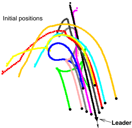
Figure 10: Trace of the vehicles while forming and keeping the spread formation with ten vehicles. Note the circular trajectory of the vehicles at the beginning, while trying to align the formation with the course of the leader.
