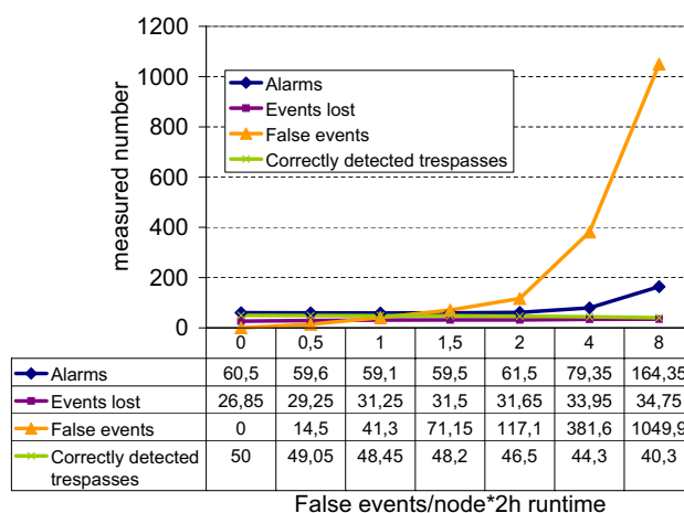
Fig. 5. Influence of false events on trespass detection
