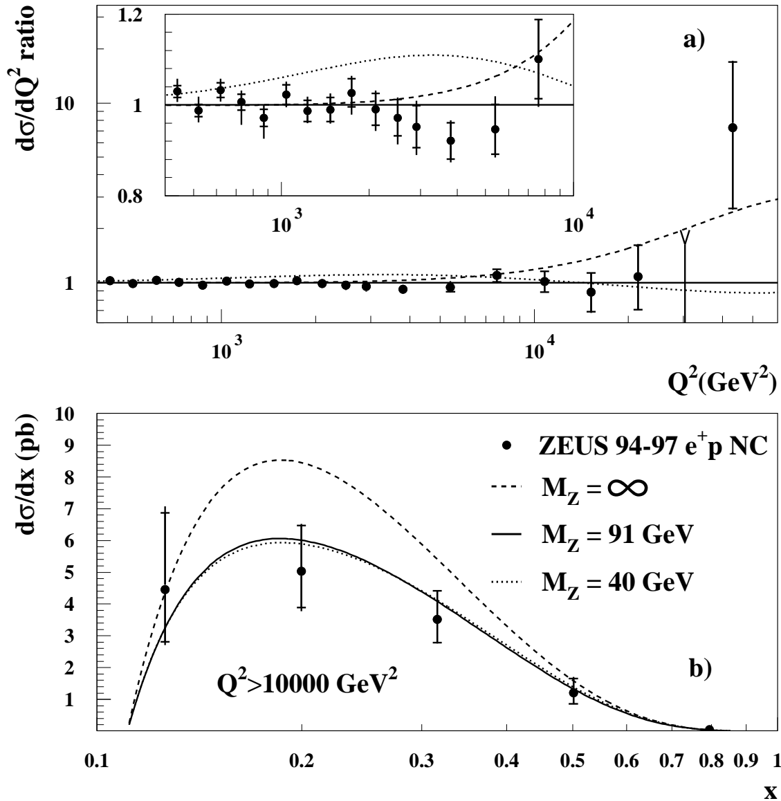
Figure 8: The points with error bars give the ratio of the measured cross-sections, d\sigma/dQ^2 , to the SM prediction using the CTEQ4D parton momentum distributions and fixing the Z^0 mass, M_Z , at its nominal value of 91.175 GeV (a) and d\sigma/dx for Q^2 > 10000 GeV 2 (b). The three lines show the SM predictions for M_Z = 91.175 GeV (solid line), for M_Z = 40 GeV (dotted line) and for no Z^0 contribution (dashed line). The inner error bars (delimited by the horizontal lines) show the statistical errors, the outer ones the statistical and systematic uncertainties added in quadrature.
