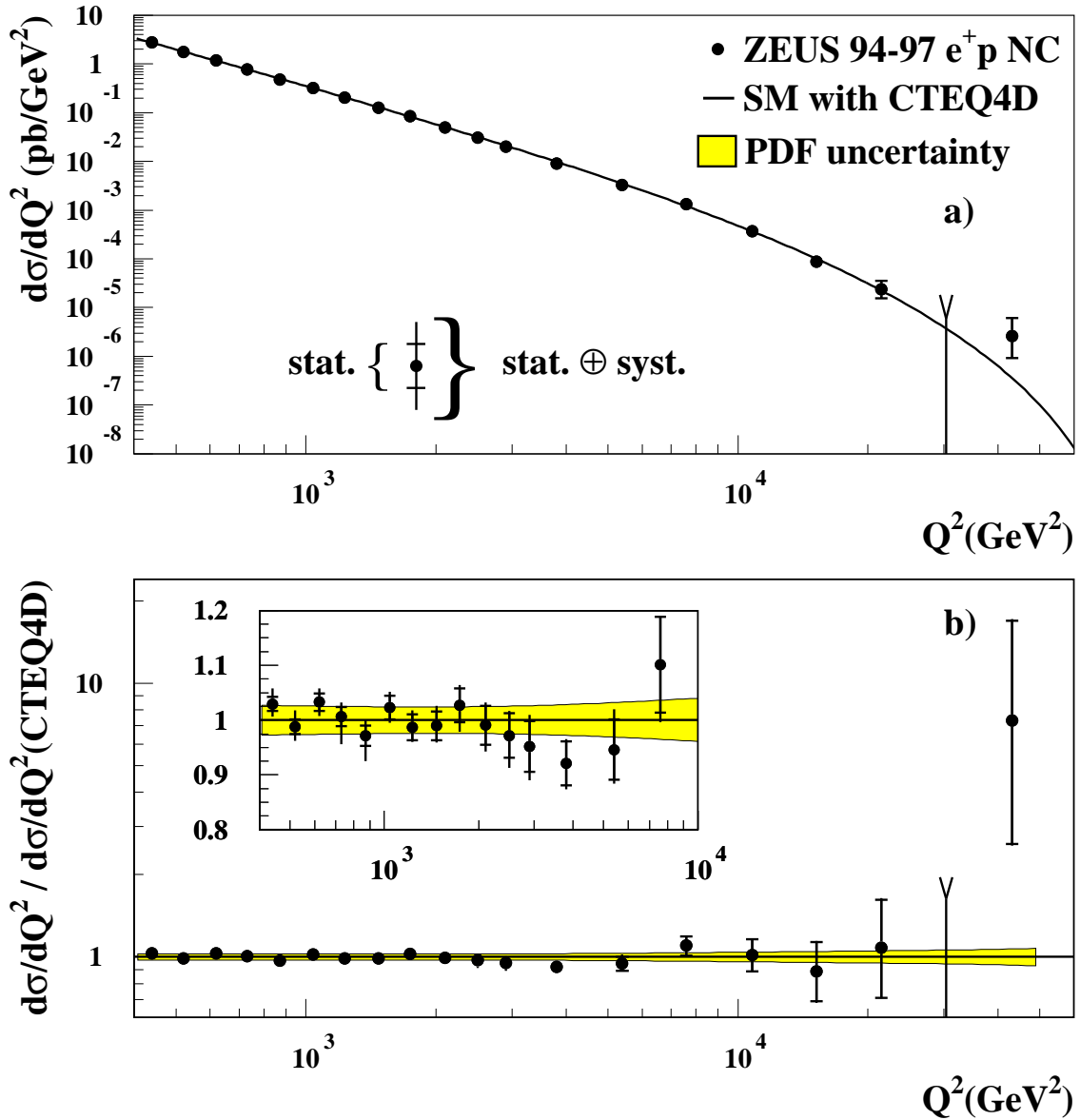
Figure 5: The high- Q^2 e^+p NC DIS cross-section, d\sigma/dQ^2 , for data (points with error bars) and the Standard Model predictions using the CTEQ4D parton momentum distributions (a). Also plotted is the ratio of data to the prediction (b). The inner error bars (delimited by the horizontal lines) show the statistical errors, the outer ones the statistical and systematic uncertainties added in quadrature. The shaded region gives the uncertainty in the Standard Model prediction due to the uncertainty in the parton momentum distributions (PDF) [20].
