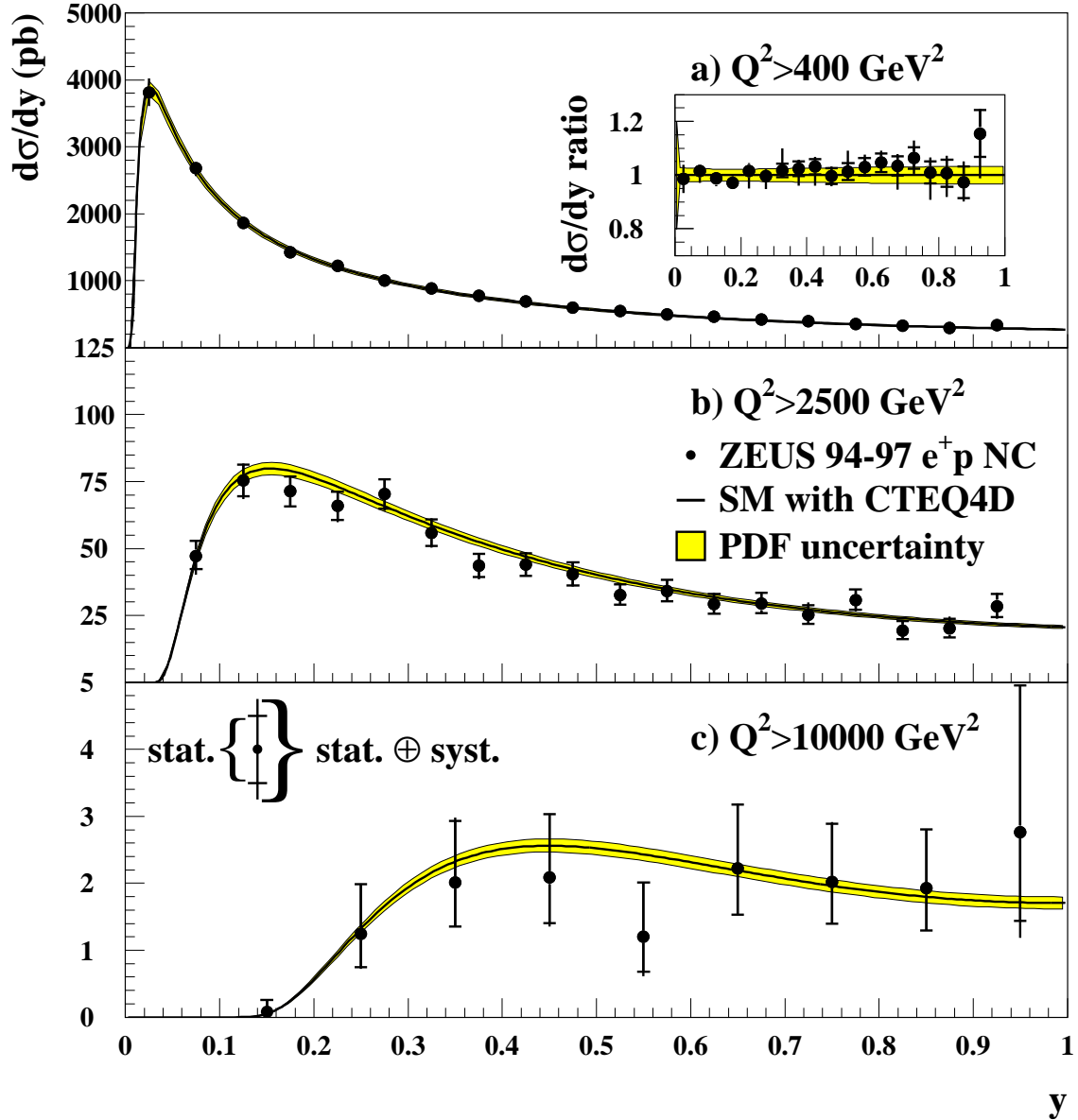
Figure 7: The high- Q^2 e^+p NC DIS cross-section, d\sigma/dy , for data (points with error bars) and the Standard Model predictions using the CTEQ4D parton momentum distributions. Plotted are cross-sections for (a) Q^2 > 400 \text{ GeV}^2 , (b) Q^2 > 2500 \text{ GeV}^2 , and (c) Q^2 > 10000 \text{ GeV}^2 . The inner error bars (delimited by the horizontal lines) show the statistical errors, the outer ones the statistical and systematic uncertainties added in quadrature. The shaded region gives the uncertainty in the Standard Model prediction due to the uncertainty in the parton momentum distributions (PDF) [20]. The inset in (a) shows the ratio of data to the prediction.
