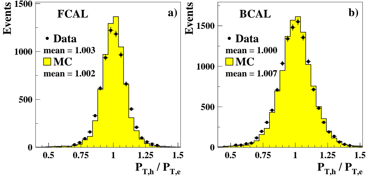
Figure 3: A comparison of data (dots) and MC (histogram) for the ratio of the transverse momentum of the hadronic final state, P_{T,h} , and the positron, P_{T,e} , for P_{T,h} > 20 GeV and \gamma_h pointing into the FCAL (a) and into the BCAL (b).
