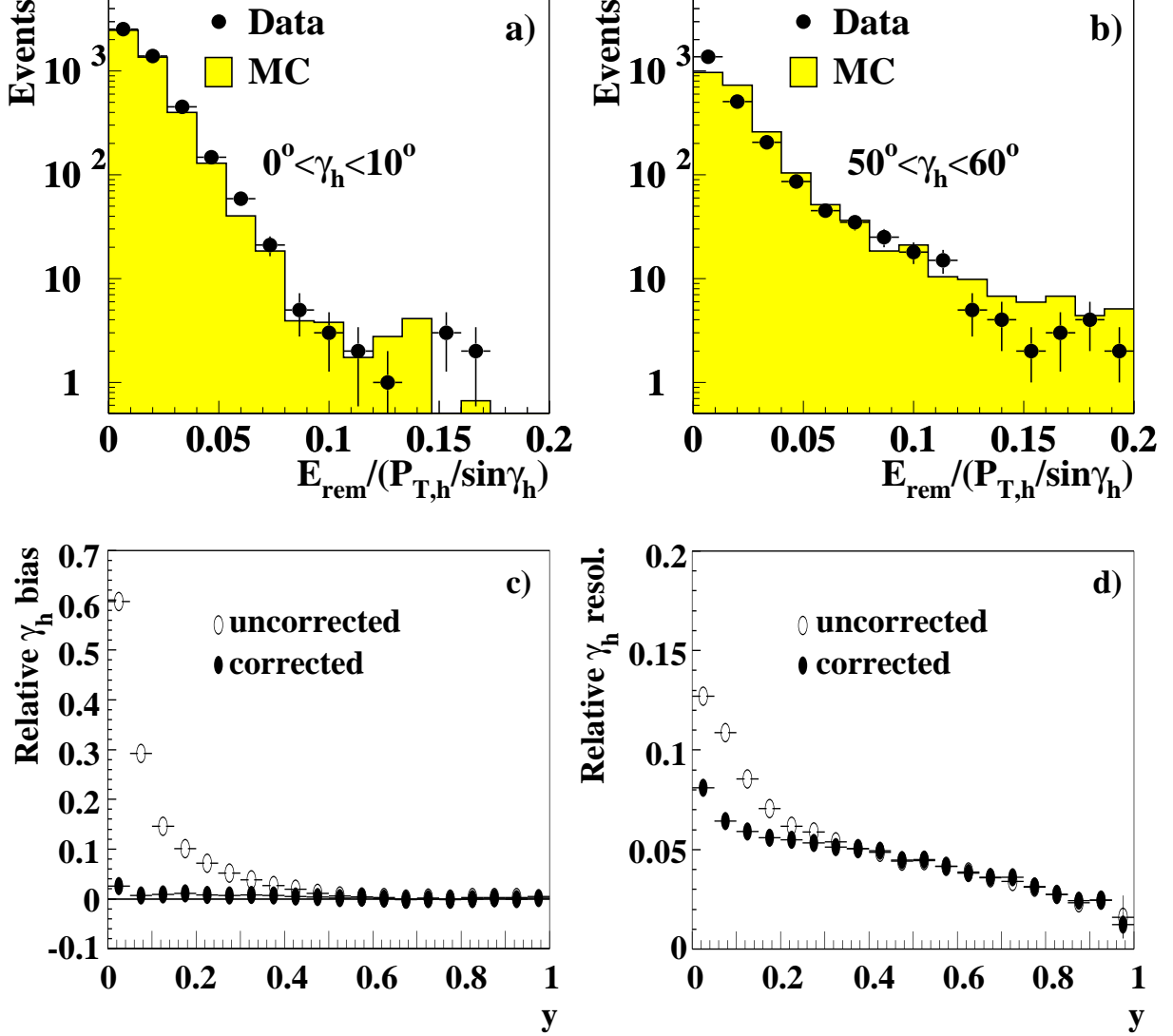
Figure 1: The effect of the correction used for the reconstruction of the angle \gamma_h as described in Section 5.4. (a) and (b): the ratio of total energy E_{\text{rem}} removed by the correction and the hadronic transverse momentum P_{T,h} divided by \sin \gamma_h for two different ranges in \gamma_h . The improvement in the reconstruction of \gamma_h by applying the correction is shown for the relative bias in \gamma_h (c) and the relative resolution in \gamma_h (d), where relative refers to the normalization to the true \gamma ; both are shown as a function of the true y as defined in Eq. (11). The result with (without) correction as obtained from a NC MC is shown as filled (unfilled) symbols.
