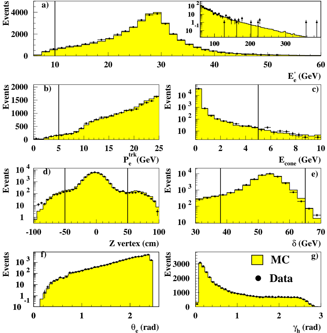
Figure 4: A comparison of data (points) and the signal MC predictions (histograms) for (a) E'_e , the energy of the scattered positron; the inset shows the high energy part of the distribution; (b) P_e^{\text{trk}} , the momentum of the positron track; (c) the energy E_{\text{cone}} not assigned to the positron in an \eta - \Phi cone of 0.8; (d) the Z position of the event vertex; (e) \delta = \Sigma(E_i - p_{zi}) ; (f) \theta_e , the angle of the positron; and (g) \gamma_h , the angle of the hadronic system. Only events which pass all event selection cuts are plotted in (e) and (f); in (a)–(e), events are plotted which pass all other event selection cuts except those on the variable displayed; the cuts to be applied to this variable are indicated by the vertical lines.
