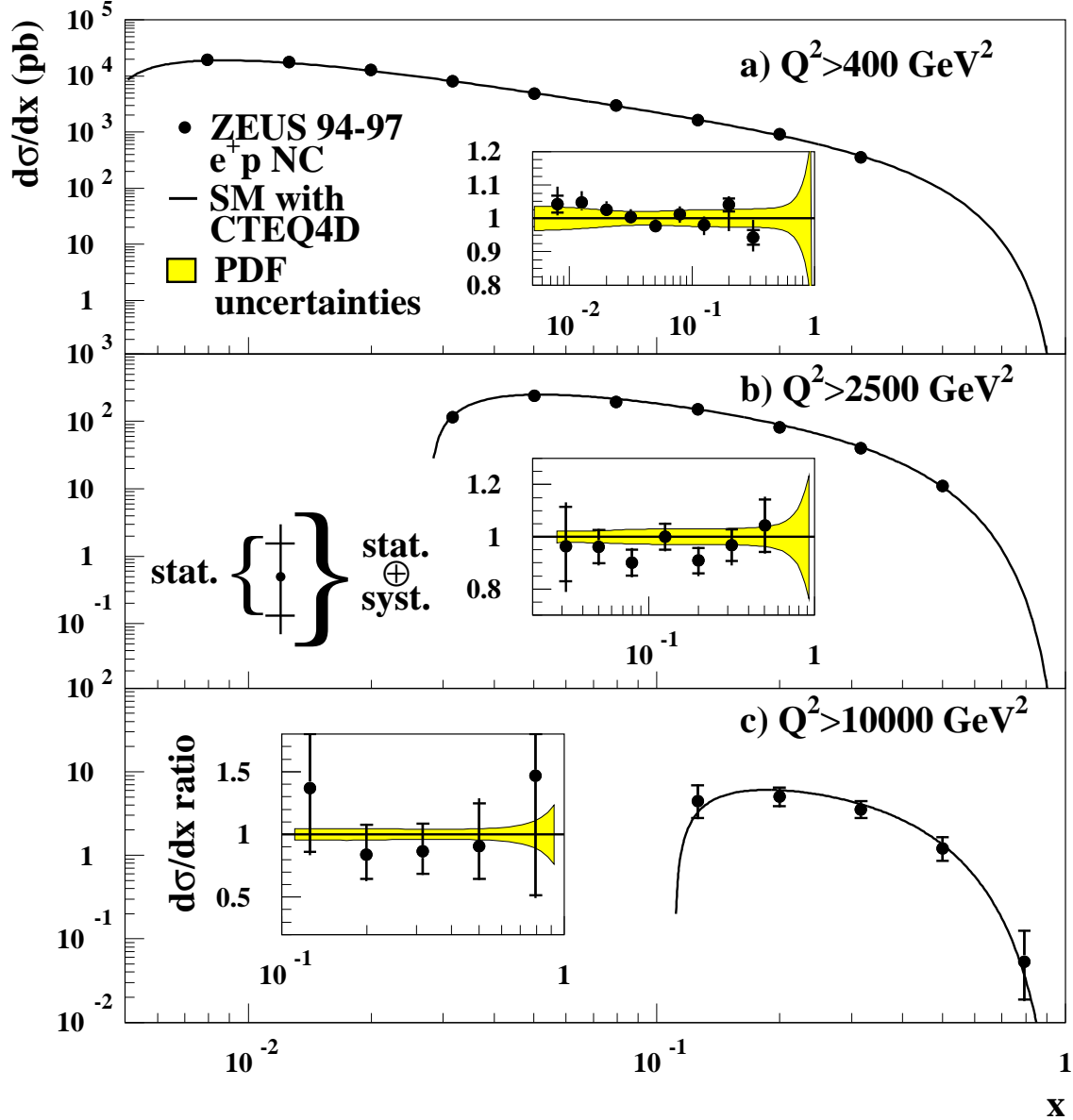
Figure 6: The high- Q^2 e^+p NC DIS cross-section, d\sigma/dx , for data (points with error bars) and the Standard Model predictions using the CTEQ4D parton momentum distributions. Plotted are cross-sections for (a) Q^2 > 400 \text{ GeV}^2 , (b) Q^2 > 2500 \text{ GeV}^2 , and (c) Q^2 > 10000 \text{ GeV}^2 . The inner error bars (delimited by the horizontal lines) show the statistical errors, the outer ones the statistical and systematic uncertainties added in quadrature. The shaded region gives the uncertainty in the Standard Model prediction due to the uncertainty in the parton momentum distributions (PDF) [20]. The insets show the ratio of data to the prediction.
