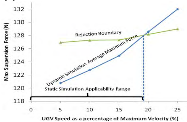
Figure 13: Statistical test for comparison of dynamic and static simulations for \omega_r=4 , \Delta =
