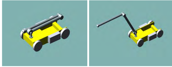
Figure 2: Multi-body dynamic simulation model in the “closed-in” position and the “manipulator extended” position
