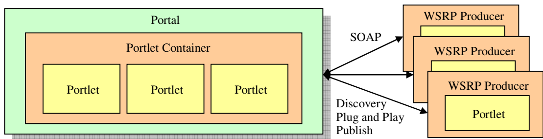
Figure 2: WSRP 1.0 defines contract for portlet containers to exchange information.
