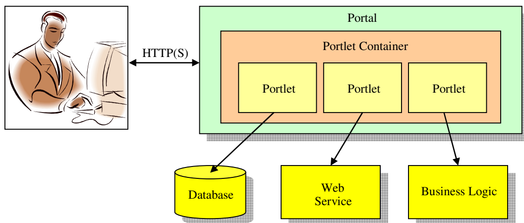
Figure 1: JSR 168 defines standard between portlets and portlet container.
