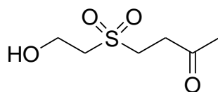
Figure 1. Chemical structure of dihydroaustrasulfone alcohol.
