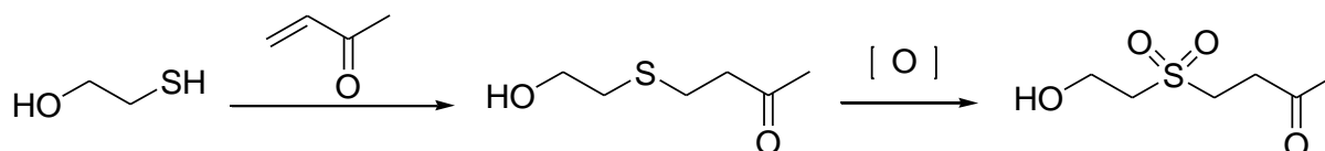
Scheme 1. Synthetic sequence of dihydroaustrasulfone alcohol.
