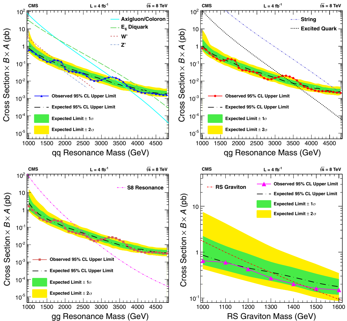
FIG. 2 (color online). Observed upper limits at 95% C.L. on \sigma \times B \times A for resonances decaying to qq , qg , and gg final state (points and solid lines) compared with the expected limits (dot-dashed dark lines) and their variation at the 1\sigma and 2\sigma levels (shaded bands). Predicted cross sections for various resonance assumptions are shown. The signal shape for the RS model is obtained by weighting the shapes for qq and gg final states according to LO calculations of the relative branching fractions.
