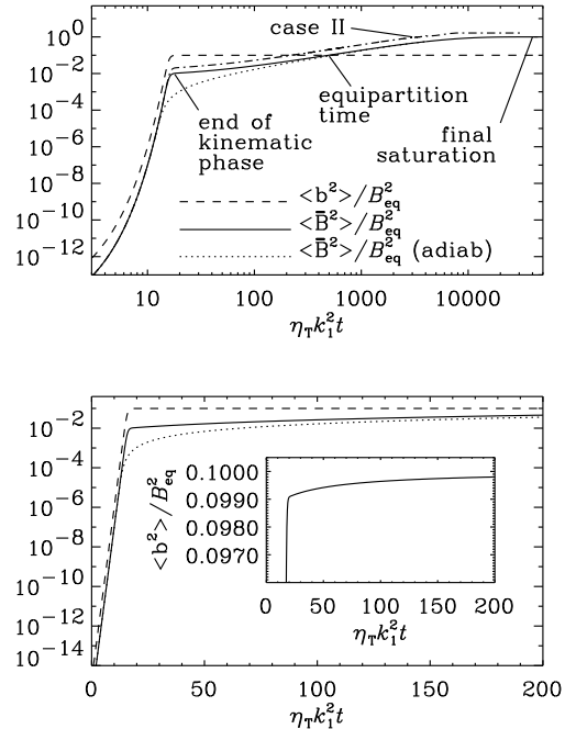
Fig. 1.— The upper panel shows the evolution of the dimensionless \langle \bar{\mathbf{B}}^2 \rangle and \langle \mathbf{b}^2 \rangle (solid and dashed lines, respectively, and both in units of B_{\text{eq}}^2 ) in a doubly-logarithmic plot for an \alpha^2 dynamo with \eta_t = \text{const} (case I). The adiabatic approximation gives significantly smaller values of \langle \bar{\mathbf{B}}^2 \rangle by the end of the kinematic growth phase. The dash-dotted line gives \langle \bar{\mathbf{B}}^2 \rangle for case II ( \eta_t \propto \alpha ); \langle \mathbf{b}^2 \rangle is essentially the same in cases I and II. Note that time is displayed on a logarithmic scale to accommodate comfortably both the kinematic phase and the final saturation. The lower panel gives the same three curves in a semi-logarithmic plot. The inset shows the slow and small ( \sim 1\% ) adjustment of \langle \mathbf{b}^2 \rangle during the early saturation phase. R_m = 10^4 , C_\alpha = 2 , C_\Omega = 0 , \kappa_f = 10 , \epsilon_f = 1 , \tilde{g} = 0 .
