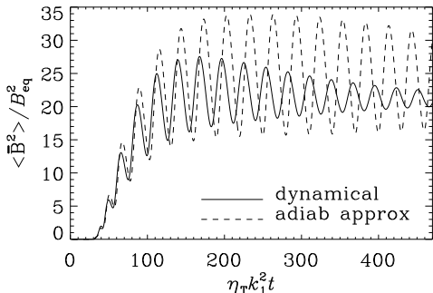
Fig. 5.— Evolution of the large scale magnetic energy for Model AG2 (solid line). The dotted line gives the comparison with the corresponding adiabatic approximation (see appendix A). R_m = 100 , C_\alpha = 0.5 , C_\Omega = 20 , \kappa_f = 5 , \epsilon_f = 1 , \tilde{g} = 3 .
