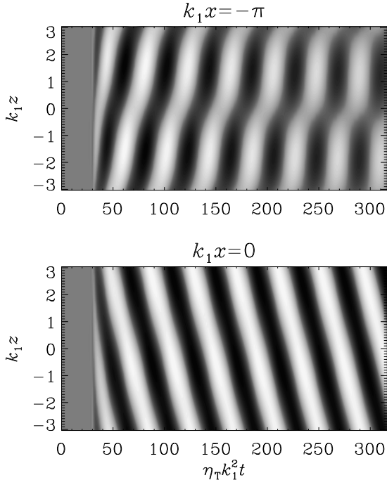
Fig. 4.— Space-time (or butterfly) diagram of \overline{B}_y for Model S1 with dynamical quenching. At x = -\pi ( x = 0 ) the shear has attained and negative (positive) maximum. Dark (light) shades indicate negative (positive) values. R_m = 30 , C_\alpha = 0.35 , C_\Omega = 33 , \kappa_f = 5 , \epsilon_f = 1 , \tilde{g} = 3 .
