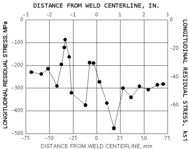
Fig. 19 – Longitudinal residual stress distribution across a flash butt welded induction-hardened railroad rail head.
