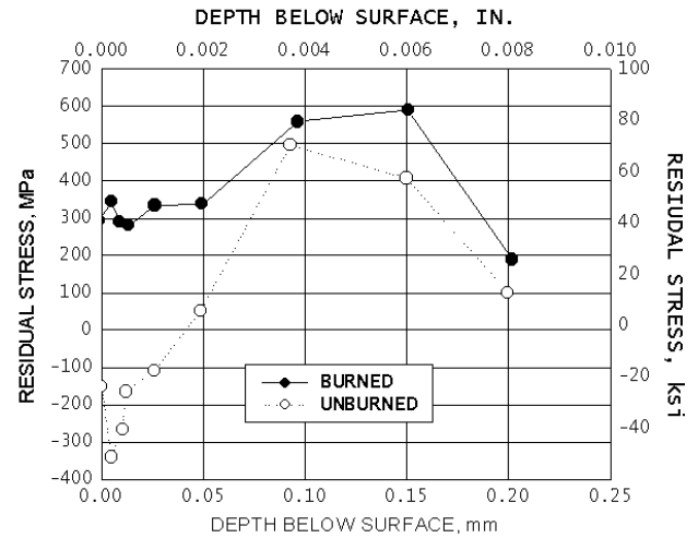
Fig. 18 – Subsurface residual stress profiles produced in burned and unburned regions of abusively ground 4340 alloy steel (50 HRC)
