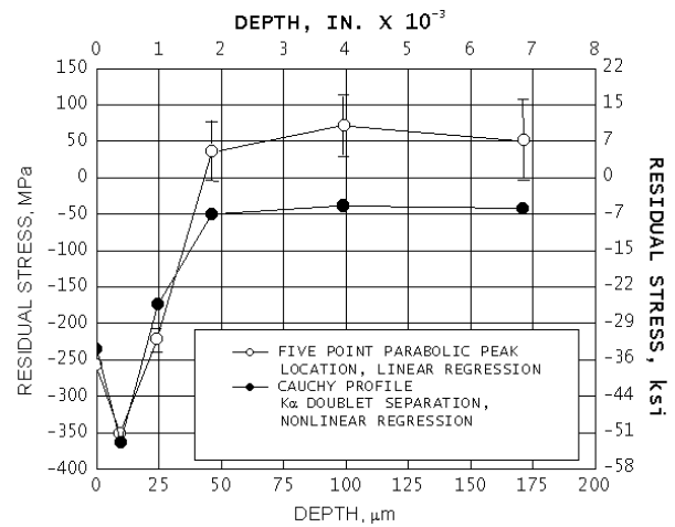
Fig. 7 -Comparison of residual stress patterns derived using Cauchy and parabolic peak location for a ground Ti-6Al-4V sample using a six-angle \sin^2\psi technique. Errors in stress measurement by two methods of diffraction-peak location are shown.
