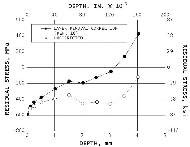
Fig. 12 -Longitudinal residual stress distribution with and without correction for removal of the carburized case from a 16-mm (5/8-in.) diam 1070 steel shaft
