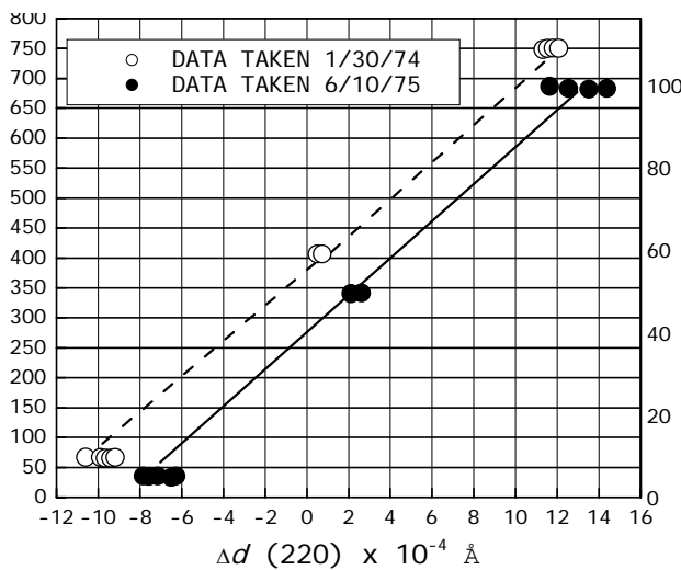
Fig. 10 -X-ray elastic constant determination for Inconel 718, (220) planes \Delta\psi = 45^\circ d_0 = 1.1272 \text{ \AA}
