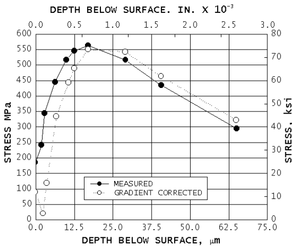
Fig. 11 – Effect of the stress gradient correction on the measurement of near-surface stresses for ground 4340 steel, 50 HRC
