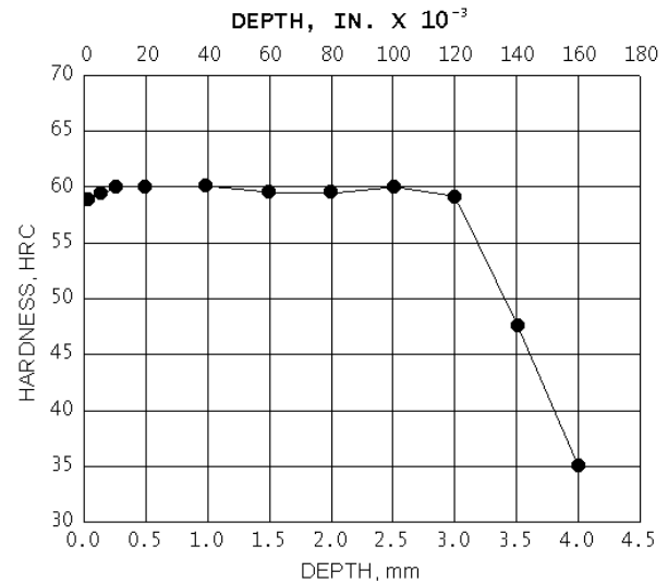
Fig. 14 -Hardness (Rockwell C scale) distribution in an induction-hardened 1070 carbon steel shaft
