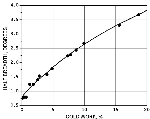
Fig. 9 -Diffraction-peak breadth at half height for the (420) peak for Rene 95 as a function of cold-working percentage
