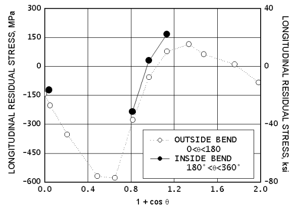
Fig. 16 -Longitudinal residual stress as a function of the quantity (1 + \cos \theta) for a 63-mm (2.5-in.) Inconel 600 U-bend
