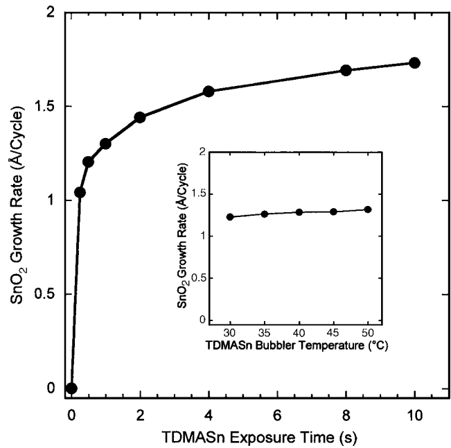
FIG. 3. \text{SnO}_2 growth rate vs TDMASn exposure time measured using ellipsometry for films deposited on Si(100) with the timing sequence x:5:1:5 at 175^\circ\text{C} . Inset shows the effect of varying the TDMASn bubbler temperature on the \text{SnO}_2 growth rate using the timing sequence 1:5:1:5.
