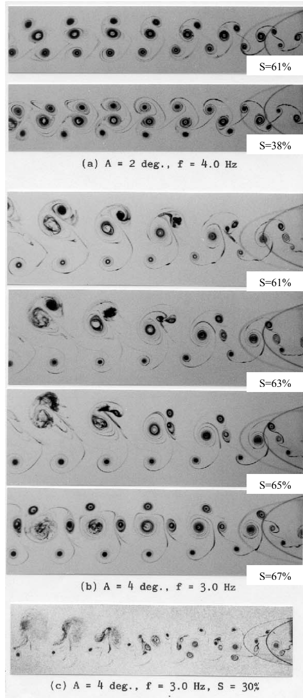
Fig. 7 Wake patterns for nonsinusoidal oscillation waveform.
