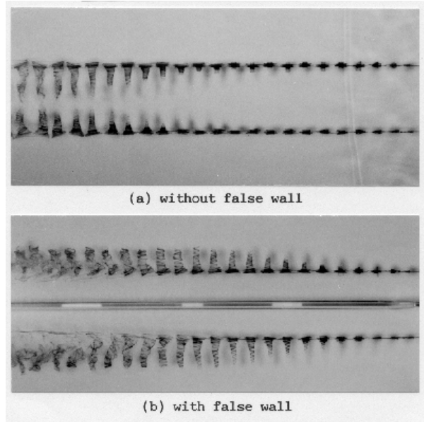
Fig. 12 Effect of a false wall on the axial flow in the vortex cores, A \approx 2 deg, f = 4.0 Hz, sinusoidal oscillation.
