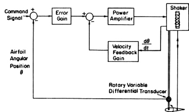
Fig. 1 Schematic of servosystem for control of airfoil angular position.
