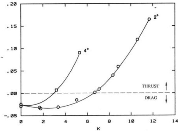
Fig. 6 Variation of force coefficient with reduced frequency.
