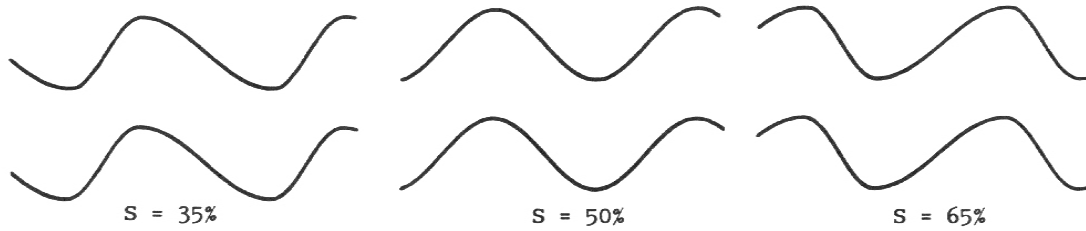
Fig. 2 Examples of pitch waveforms. Upper trace: airfoil angular position. Lower trace: command signal.
