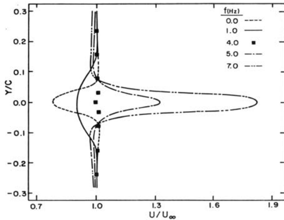
Fig. 5 Mean velocity profiles in the wake of a sinusoidally pitching NACA 0012 airfoil ( X/C = 1 ), A = 2 deg.
