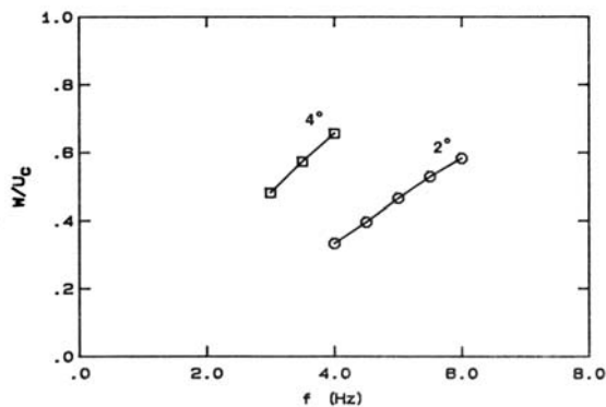
Fig. 11 Estimated axial velocity in the vortex cores.
