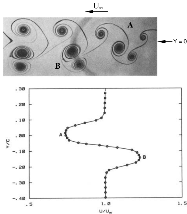
Fig. 8 Mean velocity profile at X/C = 1 for the case A = 2 deg., f = 4.0 Hz, s = 38\% , and the corresponding vortex arrangement.
