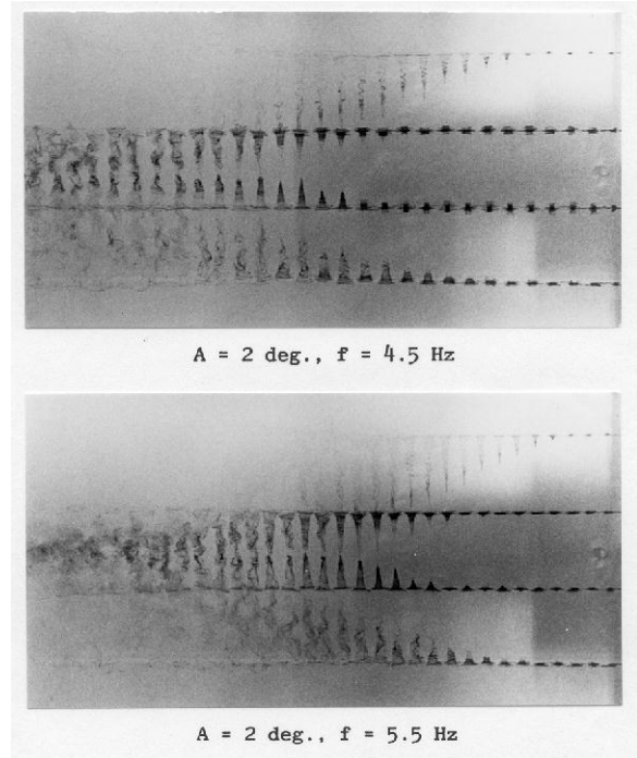
Fig. 9 Plan view showing the axial flow in the vortex cores (sinusoidal oscillation). Flow is from right to left. Right edge of photographs coincides with airfoil trailing edge.
