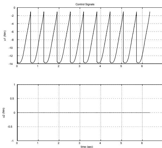
Figure 6: Control signals
