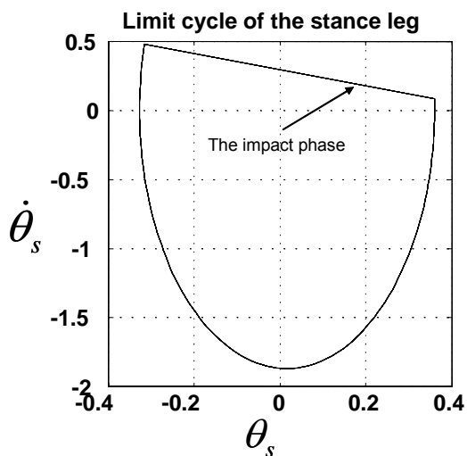
Figure 4: Passive limit cycle of the stance leg
