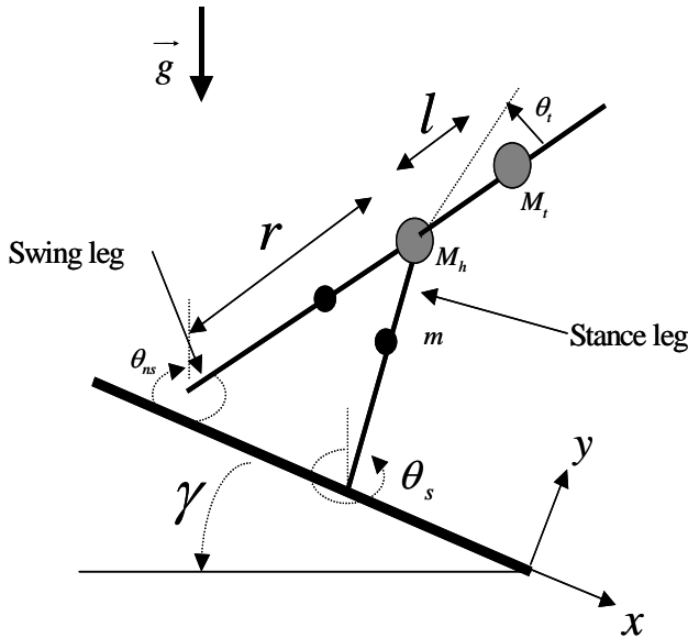
Figure 1: A passive dynamic walking model of the biped robot with torso
