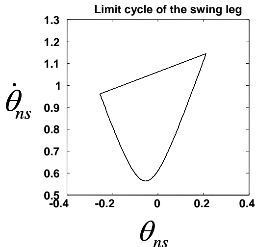
Figure 5: Passive limit cycle of the swing leg
