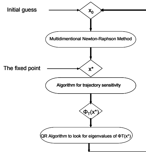
Figure 3: Algorithm for the numerical analysis
