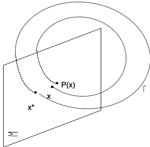
Figure 2: Poincaré Map
