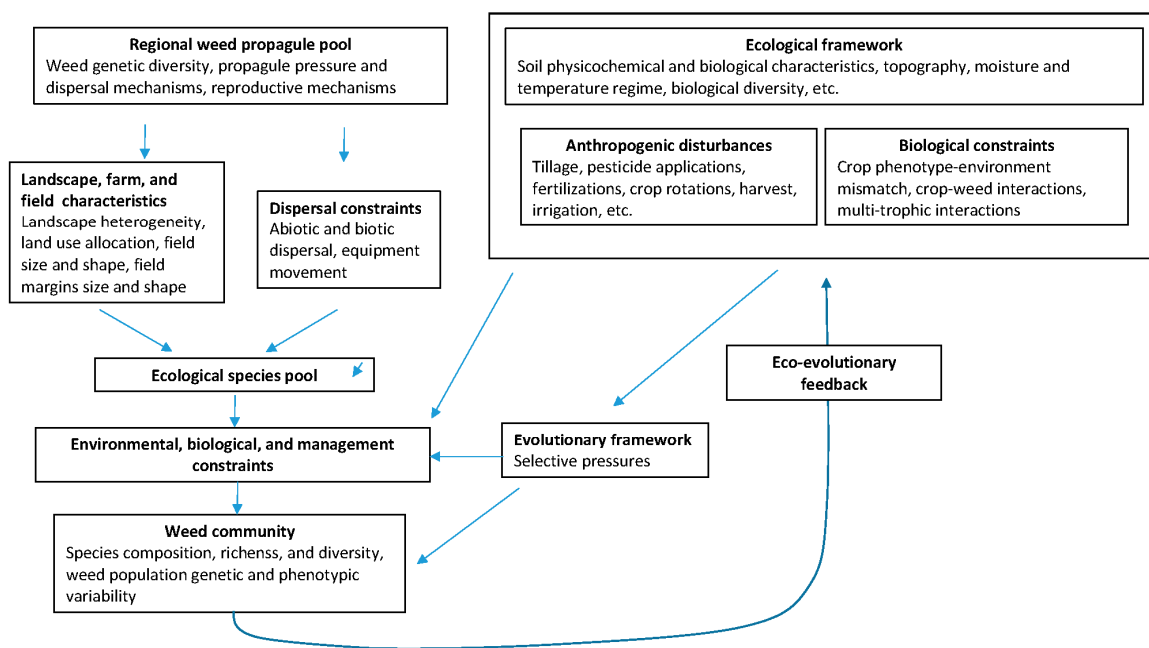
Figure 1. The eco-evolutionary conceptual framework determining the selective pressures determining the characteristic of the weed community and the resulting eco-evolutionary feedback. The left panel of this figure is adapted from Booth and Swanton, and Petit et al.
