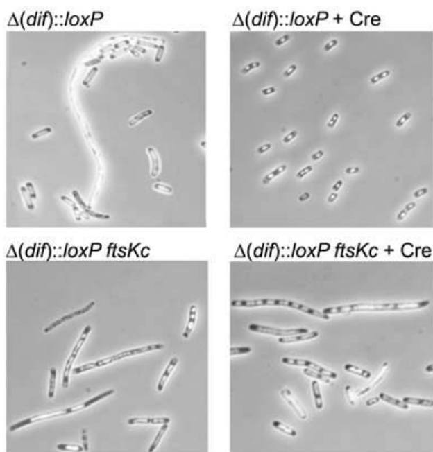
Fig. 4. Phase-contrast fluorescence micrographs of strains carrying the loxP site in place of dif (DAPI staining). Top left, FC149 [LN2666 \Delta(dif)::Tc::loxP -Kn- loxP ]; top right, FC149/pFX71; bottom left, FC407 (FC149 ftsKc ::Cm); bottom right, FC407/pFX71.
