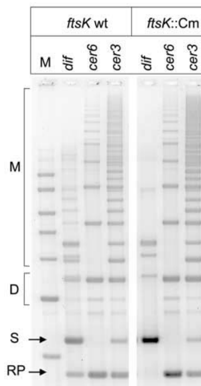
Fig. 3. Recombination between plasmid-borne core sequences. Strains FX55 ( ftsK wt) and FX60 (FX55 ftsK::Cm ) were transformed with plasmids containing direct repetitions of the core sequences: pBH220 ( dif ), pBH222 ( cer6 ) or pBH223 ( cer3 ). Plasmid DNA was recovered after overnight growth and analysed by agarose gel electrophoresis. Positions of the substrate (S), the recombination product containing one core sequence (RP) dimers of S and RP (D), and higher multimers (M) formed by Xer recombination are indicated on the left. Note the disappearance of the forms corresponding to plasmids carrying the initial repetition of cer6 due to a higher rate of recombination at cer6 than at cer3 and dif .
