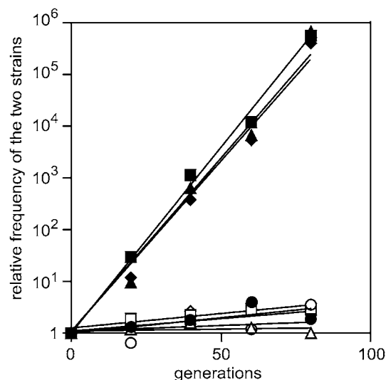
Fig. 5. Viability defect due to inactivation of dif and FtsKc. Strains LN2666 (wt), FC126 [ \Delta(dif)2600::Gm ], FC405 ( ftsK ::Cm) and FC318 [ \Delta(dif)2600::Gm ftsK ::Cm] were mixed by pairs and grown in serial culture. Closed symbols, LN2666 versus each mutant strain. The relative frequency of LN2666 is plotted. Diamonds, LN2666 versus FC126; squares, LN2666 versus FC405; triangles, LN2666 versus FC318; circles, FC232 (LN2666 recA56 ) versus FC420 [ \Delta(dif) ftsK ::Cm recA56 ]. Open symbols: mutant strain versus mutant strain. The frequency of the first strain cited is plotted. Diamonds, FC126 versus FC318; squares, FC126 versus FC405; circles, FC405 versus FC318; triangles (control), FC126 versus LN3079 [ \Delta(dif)2600::Tc ].
