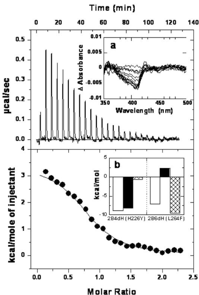
Fig. 5. Calorimetric titration profile (upper panel) and the resulting integrated binding enthalpy data of 1-BI binding to P450 2B6dH L264F are shown. The data were fit to single-class of binding site model to obtain thermodynamic parameters. Inset a, difference spectra of 1-BI binding; inset b, the thermodynamic signatures ( \Delta G = open bars, \Delta H = filled bars, and -T\Delta S = crossed bars) of 1-BI binding between P450 2B4dH (Muralidhara et al., 2006) and 2B6dH.
