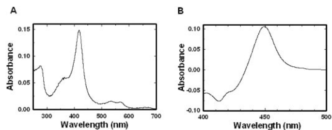
Fig. 1. Characterization of purified P450 2B6dH. A, absolute spectrum (250–700 nm). B, P450 reduced -CO difference spectrum (400–500 nm).
