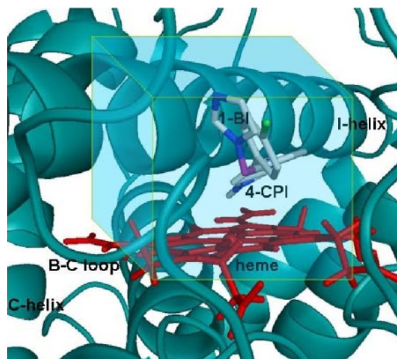
Fig. 6. Molecular docking of 1-BI and 4-CPI in the active site of a P450 2B6 homology model. A representative 1-BI and 4-CPI molecule of the lowest energy ensemble (6.17 and 6.52 kcal/mol, respectively) is shown. The point grid used for docking is shown on the heme plane. The mainframe structural loops of the binding pocket are labeled. The molecular graphic was generated using PyMol graphics ( http://pymol.sourceforge.net/ ). Molecular docking was performed using AutoDock version 3.05 as described earlier (Muralidhara et al., 2006). In brief, the 4-CPI bound P450 2B4dH structure (pdb code 1suo) was used to model P450 2B6dH using Modeler ( http://www.rwmodeler.com/ ). The root-mean-square deviation before and after the minimization using nanoscale molecular dynamics was found to be 0.094 and 0.948, respectively. The homology model was energy minimized and a 40 \times 40 \times 40 -point grid placed at the distal end of the heme was used for 1-BI and 4-CPI docking. A total of 10 unique minimum energy ensembles that exhibited <1 Å root-mean-square deviation were ranked, and a representative docking conformation of the lowest energy is presented.
