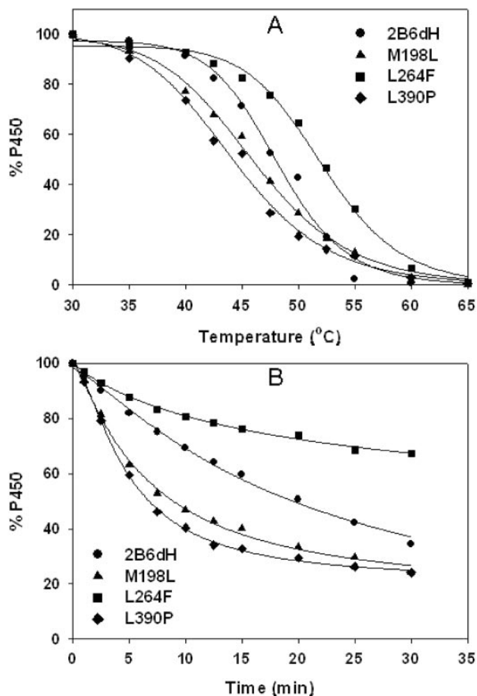
Fig. 3. A, thermal inactivation of 2B6dH mutants (1 \mu M ) monitored by a decrease in the amount of P450 as a function of temperature, as described under Materials and Methods . Determination of the total concentration of the heme protein was done by nonlinear least square approximation of the spectra by a linear combination of spectral standards of 2B4 low-spin, high-spin, and P420-states. The data were fit to a two-state transition to obtain T_m . B, time courses of inactivation of 2B6dH mutants (1 \mu M ) at 45°C monitored as described above. The data were fit to a pseudo-first-order equation to obtain k_{inact} .
