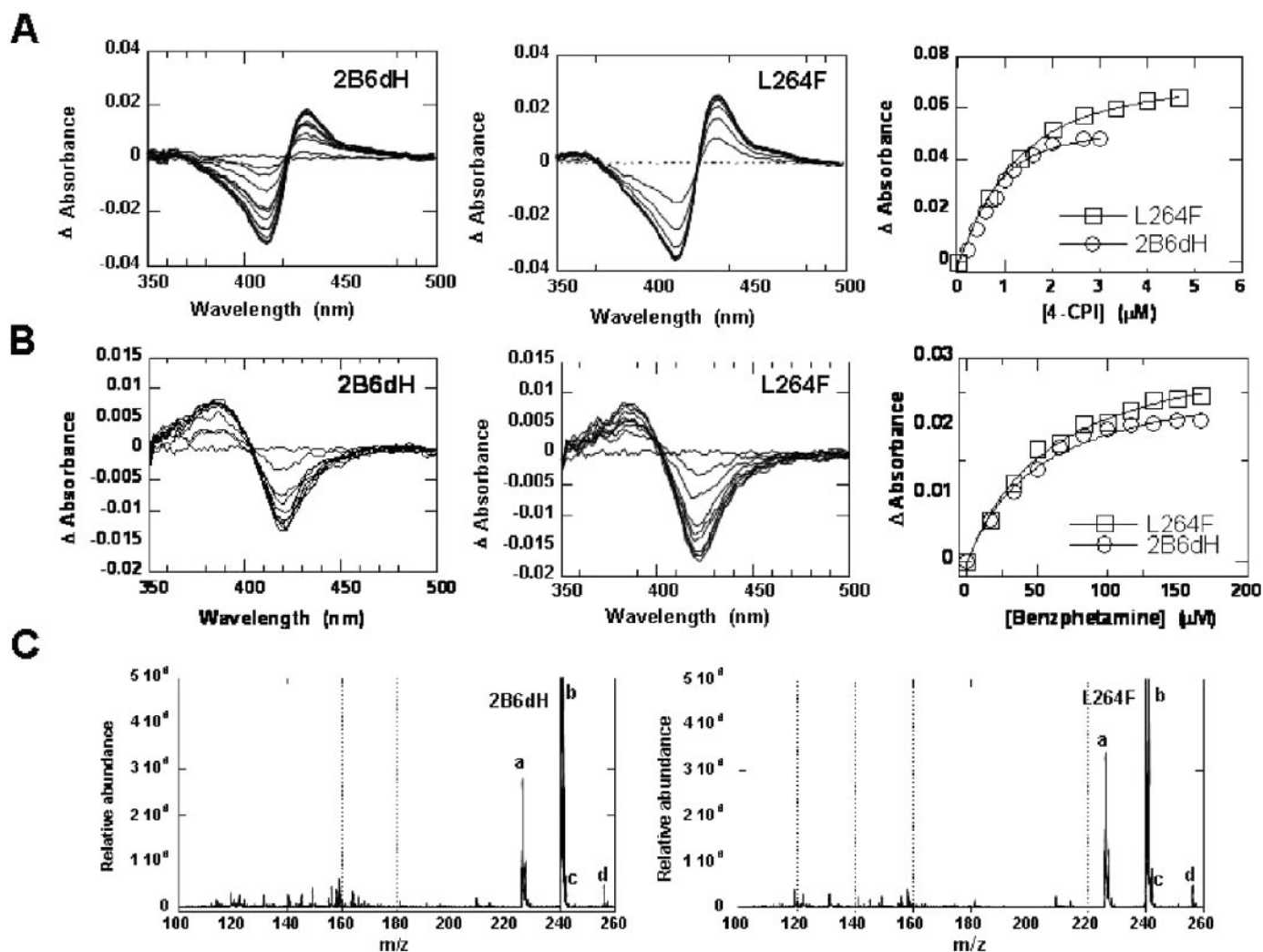
Fig. 4. Characterization of L264F. Typical type-II difference spectra of 4-CPI binding (A) and type-I spectra of benzphetamine binding (B) are shown for P450 2B6dH and L264F (left two panels). The binding data with 4-CPI (A) were fit to the tight-binding equation (2B6dH or L264F), whereas data with benzphetamine (B) were fit to the Michaelis-Menten equation, as described under Materials and Methods , to derive the K_s values as listed in Table 4. C, the LC-MS chromatogram of benzphetamine metabolites for the two proteins are shown with the peaks representing a) norbenzphetamine (mol. wt. = 226.2), b) benzphetamine (mol. wt. = 240.2), c) OH-norbenzphetamine (mol. wt. = 242.2), and d) OH-benzphetamine (mol. wt. = 256.2).
