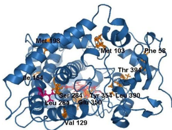
Fig. 2. Homology model of P450 2B6dH based on the crystal structure of P450 2B4 (pdb code 1SUO). The 11 residues picked for rational engineering based on the lower accessibility to bulk solvent are mapped on the structure, and the mutants created are F58L, M103V, V129L, I154V, M198L, L264F, S284H, E350D, Y354H, L390P, and T394S. The molecular graphic was generated using PyMol graphics ( http://pymol.sourceforge.net/ ).
