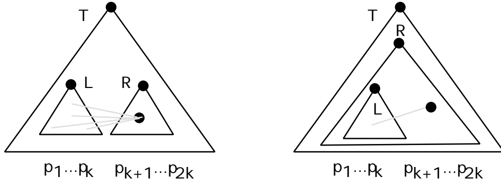
Figure 2: Two CCMG_1 Derivation Structures
