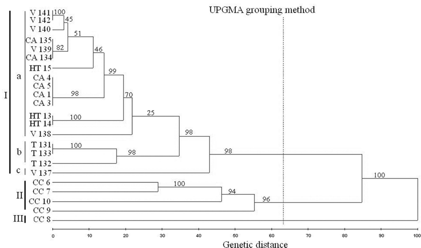
Figura 1. Dendrogram obtained by the UPGMA method from genetic distances expressed as Jaccard complements, estimated among the 23 coffee tree genotypes, based on EST-SSR markers. Cofenetic correlations: 0.98; stress: 9,1%.
