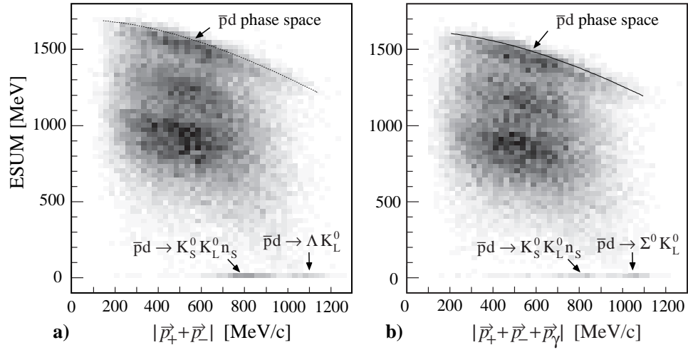
Fig. 2. a) Sum of energy deposits from photons in the electromagnetic calorimeter (ESUM) versus the total momentum of the positively and the negatively charged particles for all 2-prong events that passed the preselection criteria for \Lambda \rightarrow p\pi^- decays given in the text. b) Analogous representation of the subset satisfying the preselection criteria for \Sigma^0 \rightarrow \Lambda\gamma ( \Lambda \rightarrow p\pi^- ) decays. Here the photon attributed to this decay is excluded from ESUM.
