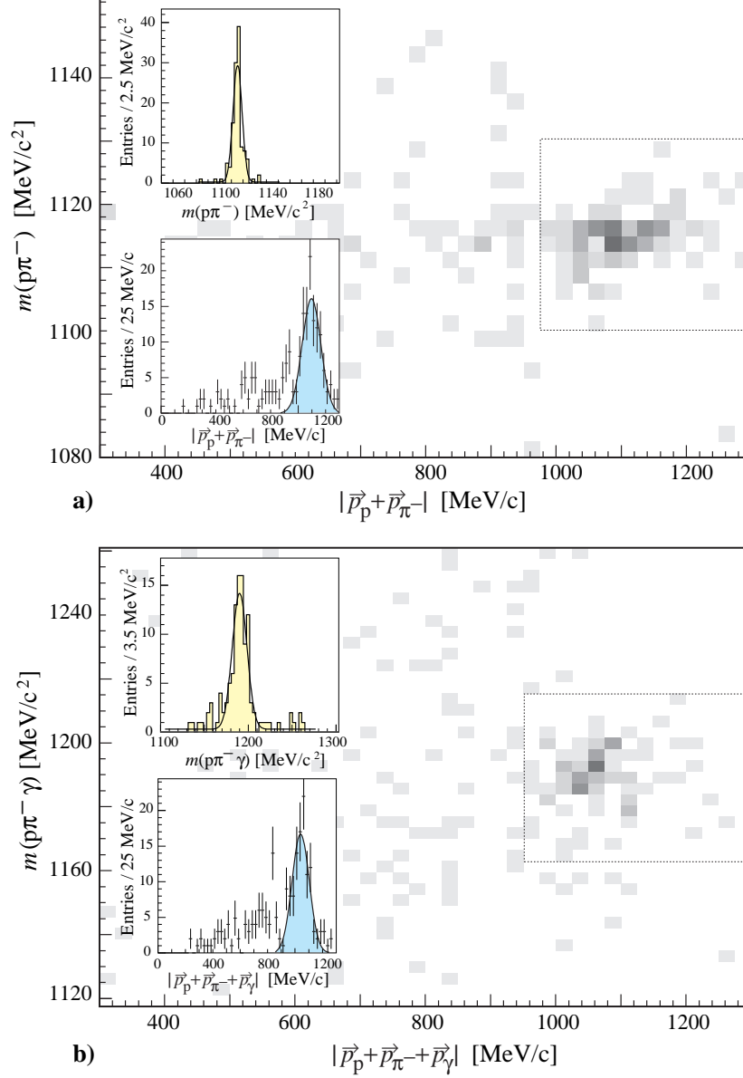
Fig. 4. a) Invariant mass versus total momentum for the p\pi^- pairs selected from Fig. 3a. The insets show the projections on both axes and Gaussian fits, yielding m(p\pi^-) = 1116 MeV/c 2 , \sigma = 4 MeV/c 2 and p = 1099 MeV/c, \sigma = 68 MeV/c. The dotted box indicates the final selection of \bar{p}d \rightarrow \Lambda K_L^0 (noninteracting) events. b) Invariant mass versus total momentum for the p\pi^-\gamma combinations, selected from Fig. 3b, and projections with Gaussian fits, yielding m(p\pi^-\gamma) = 1190 MeV/c 2 , \sigma = 8 MeV/c 2 and p = 1043 MeV/c, \sigma = 62 MeV/c. The dotted box indicates the final selection of \bar{p}d \rightarrow \Sigma^0 K_L^0 (noninteracting) events.
