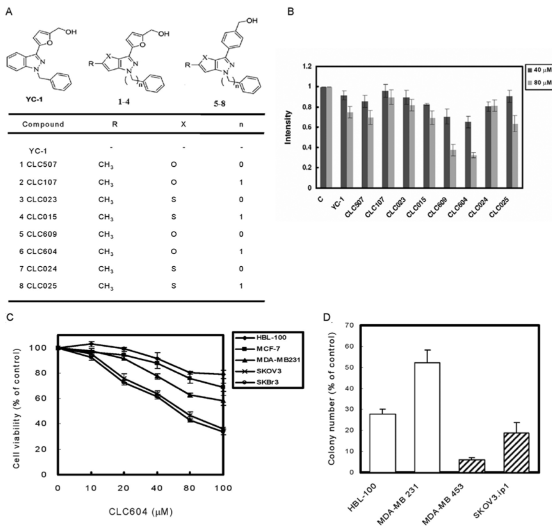
Figure 1. Effects of 1-benzyl-3-(5-hydroxymethyl-2-furyl)indazole (YC-1) and its analogues on the expression of HER2 protein. (A) Chemical structures of YC-1 and its furo-pyrazole and thienopyrazole isosteric analogues. (B) HER2-overexpressing breast cancer MDA-MB-453 cells were treated with YC-1 and its analogues (40 and 80 \mu M) at 37°C for 24 h. Immunoblotting was used to measure HER2 and \beta -actin. Changes in the protein expression of the bands were normalized to \beta -actin. Columns, mean of 3 independent experiments; bars, SD. (C) Cell viability was determined by MTT assay after continuous exposure to different concentrations of CLC604 at 37°C for 24 h. The number of viable cells after treatment is expressed as a percentage of the vehicle-only control. Data point, mean of 3 independent experiments; bars, SD. (D) Effect of CLC604 on anchorage-independent growth of cancer cells. Cells ( 1 \times 10^4 /well) were seeded in a 6-cm dish in culture medium containing 0.35% low-melting agarose over a 0.7% agarose layer in the presence of 80 \mu M of CLC604 or control vehicle and were incubated for 3 weeks at 37°C. Colonies larger than 100 \mu m were counted. The percentage of colony formation was calculated by defining the number of colonies in the absence of CLC604 as 100%. Columns, mean of 3 independent experiments; bars, SD.
