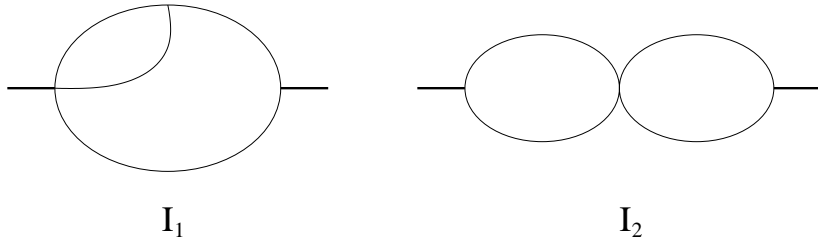
Figure 4: Divergent loop integrals
