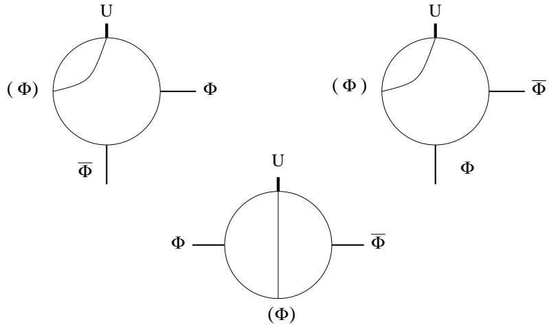
Figure 9: Two-loop contributions U(D^2\Phi)\bar{\Phi} \rightarrow B_2
