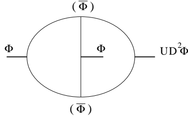
Figure 11: Two-loop contribution U(D^2\Phi)^3 \rightarrow C_1
