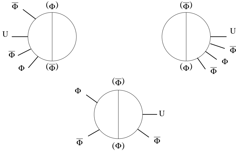
Figure 14: Two-loop contributions U(D^2\Phi)\bar{\Phi}^2 \rightarrow \tilde{C}_3
