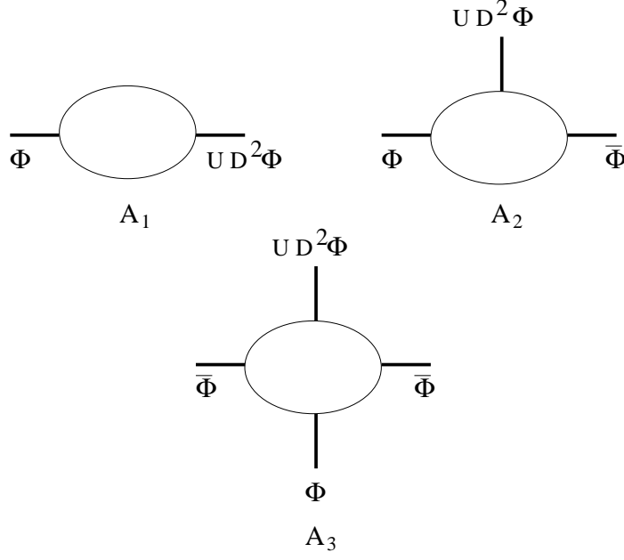
Figure 2: One-loop divergent diagrams with one insertion of the U(D^2\Phi)^3 -vertex
