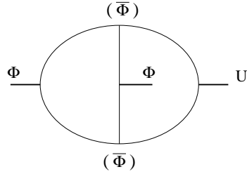
Figure 8: Two-loop contribution U(D^2\Phi)^2 \rightarrow \tilde{B}_1
