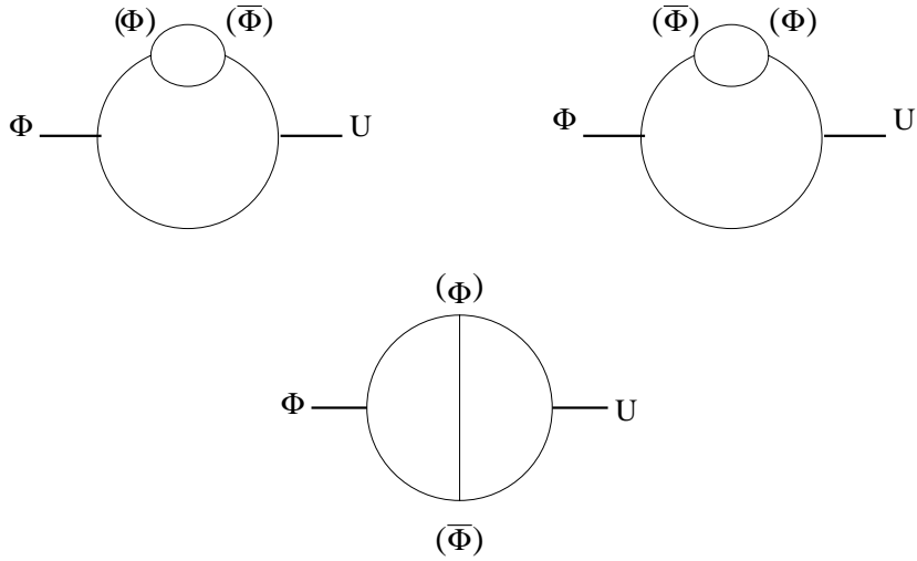
Figure 6: Two-loop contributions U(D^2\Phi) \rightarrow \tilde{T}_1
