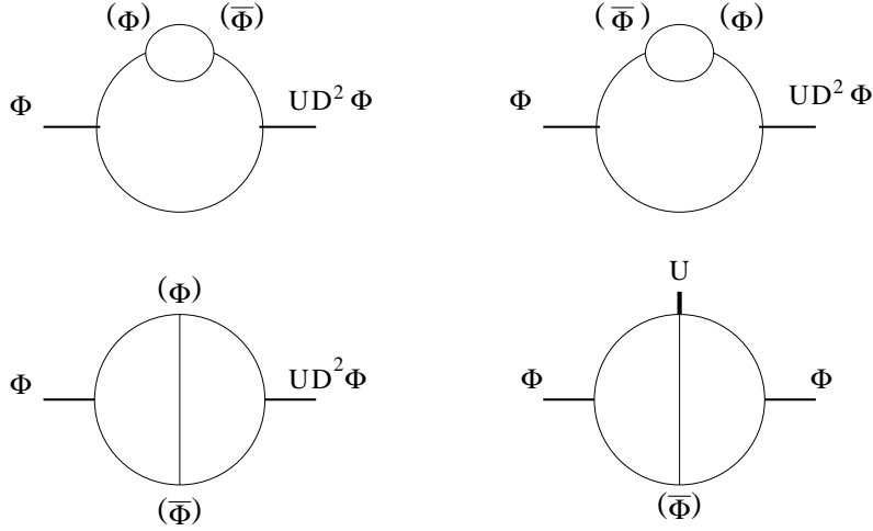
Figure 7: Two-loop contributions U(D^2\Phi)^2 \rightarrow B_1
