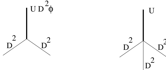
Figure 1: New vertices proportional to the external U superfield
