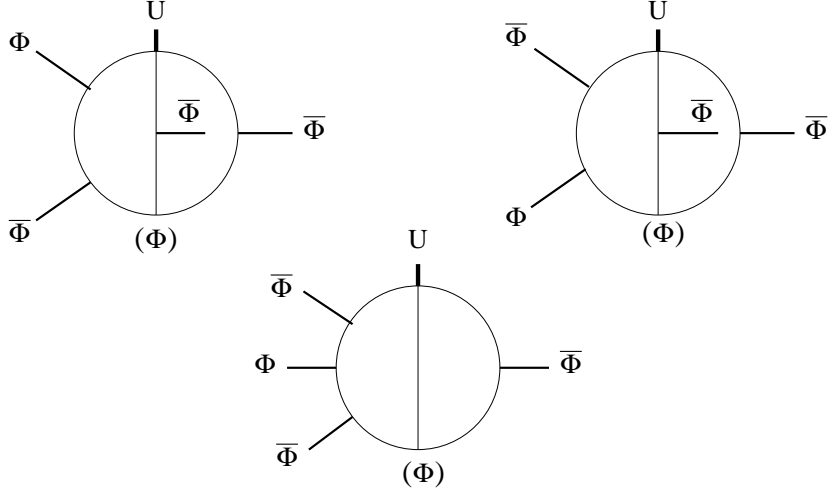
Figure 16: Two-loop contributions U(D^2\Phi)\bar{\Phi}^3 \rightarrow D_2
