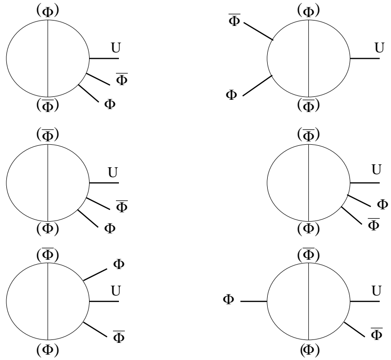
Figure 10: Two-loop contributions U(D^2\Phi)\bar{\Phi} \rightarrow \tilde{B}_2
