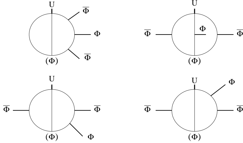
Figure 13: Two-loop contributions U(D^2\Phi)\bar{\Phi}^2 \rightarrow C_3
