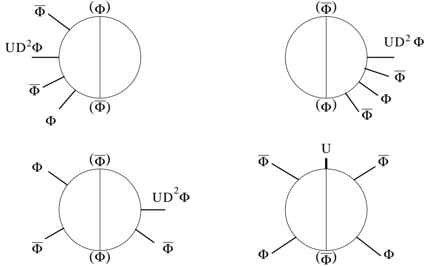
Figure 15: Two-loop contributions U(D^2\Phi)^2\bar{\Phi}^2 \rightarrow D_1
