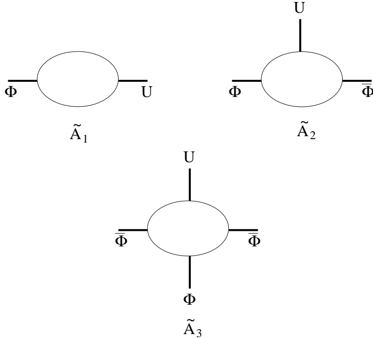
Figure 3: One-loop divergent diagrams with one insertion of the U(D^2\Phi)^2 -vertex
