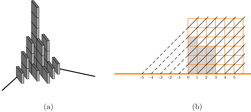
Figure 16: (a) The diagonal slicing of the plane partition: we end up with a series of 2 D partitions that obey the interlacing condition Eq(115), (b) The slices are parametrized by integers
