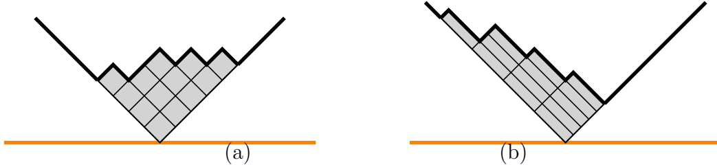
Figure 19: The profile of the partition is drawn bold; a) shows the 2D partition for the self-dual case \epsilon_2 = -\epsilon_1 , whereas b) shows the same partition for the non self-dual case \epsilon_1 \neq \epsilon_2 ( \epsilon_2 = -2\epsilon_1 )
