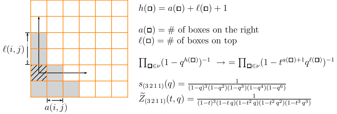
Figure 23: A Young diagram \nu = (3211) .
