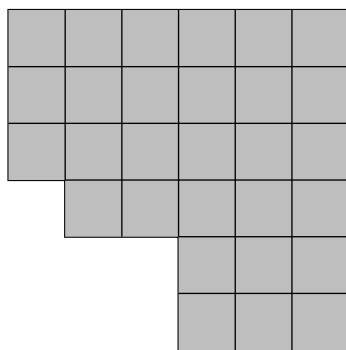
Figure 13: For a partition \lambda = \sigma(N) and an arbitrary 2D partition \nu , the skew partition \lambda/\nu is always a 2D partition, provided N \geq \max(\nu_1, \nu_1^t) .
