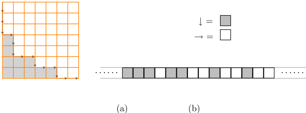
Figure 18: a) We can trace the profile of a particular 2D partition starting at j = \infty and going to i = \infty as depicted in the figure. b) To each vertical pass we associate a black box, and a white one to each horizontal pass. If we put these boxes in a row, then we get a unique “finger print” to a partition. The coordinates of the centers are given by the sets D^\pm .
