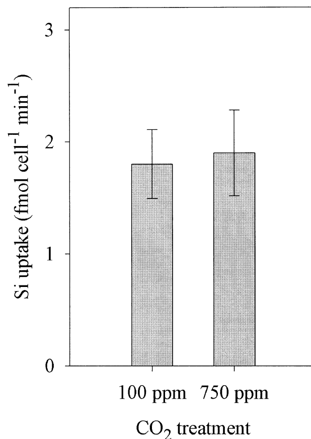
Fig. 4. Short-term (10 s) unidirectional influx rates at high and low p\text{CO}_2 from the silicon oil centrifugation technique. Error bars are 95% confidence intervals, calculated from three replicates.
