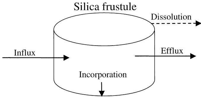
Fig. 1. Diatom silicon fluxes. Influx: the transport rate across the plasmalemma from outside to inside the cell, incorporation: the rate of frustule formation ( \text{Si cell}^{-1} \times \mu\text{-d} ), efflux: the transport rate across the plasmalemma from inside to outside the cell, dissolution: the rate of depolymerization of silica to \text{Si}(\text{OH})_4 . Loss = dissolution + efflux. Net uptake = influx – loss.
