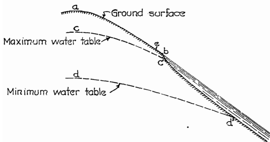
FIGURE 32.—End point of a definite stream channel
