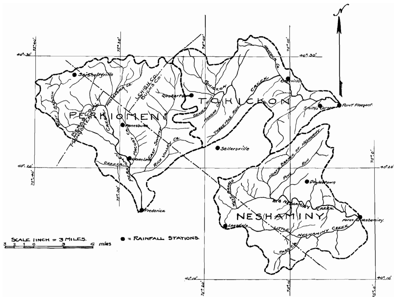
FIGURE 11.—Drainage patterns Neshaminy, Tohickon, and Perkiomen drainage basins.
