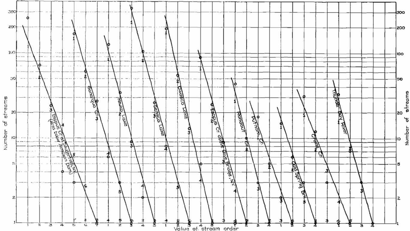
FIGURE 3.—Bifurcation or relation of stream order to number of streams in different drainage basins
