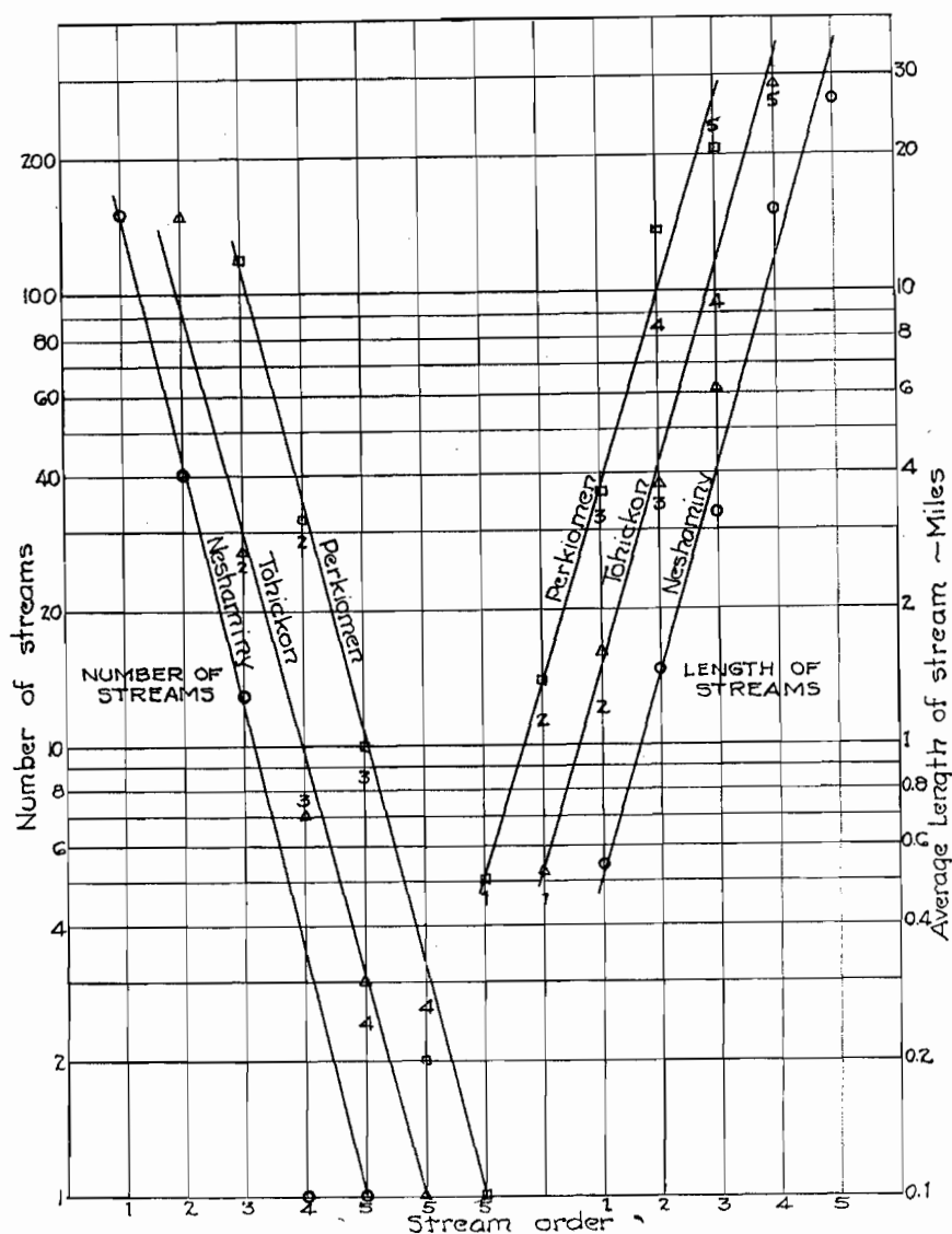
FIGURE 10.—Stream numbers and stream lengths
