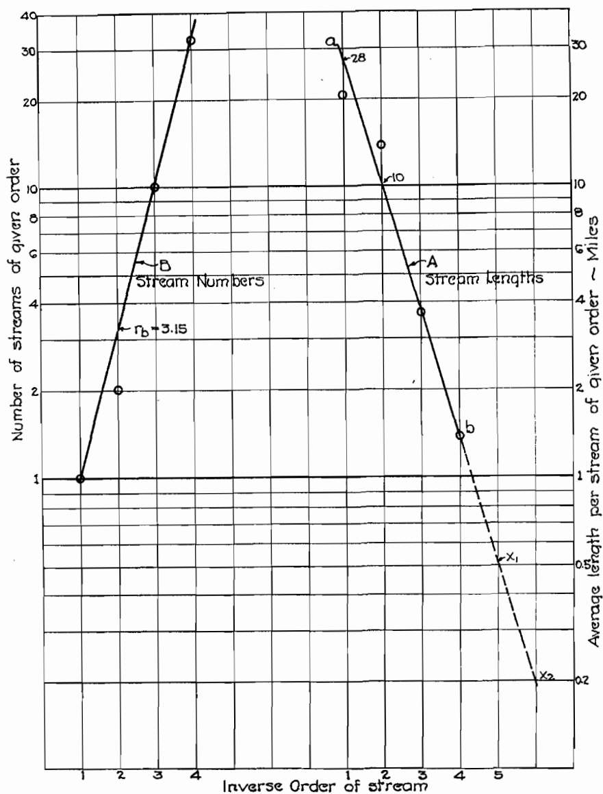
FIGURE 8.—Graphical determination of stream characteristics
