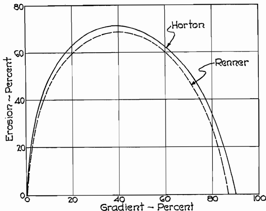
FIGURE 15.—Horton slope function for surface erosion
