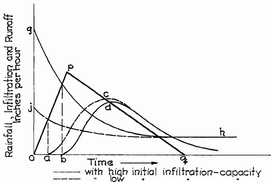
FIGURE 18.—Relation of initial infiltration-capacity to erosion
