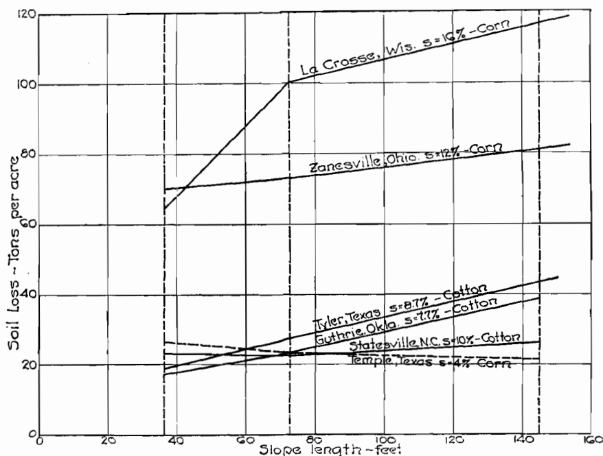
FIGURE 17.—Relation of erosion to slope length From field experiments of U. S. Soil Conservation Service.
