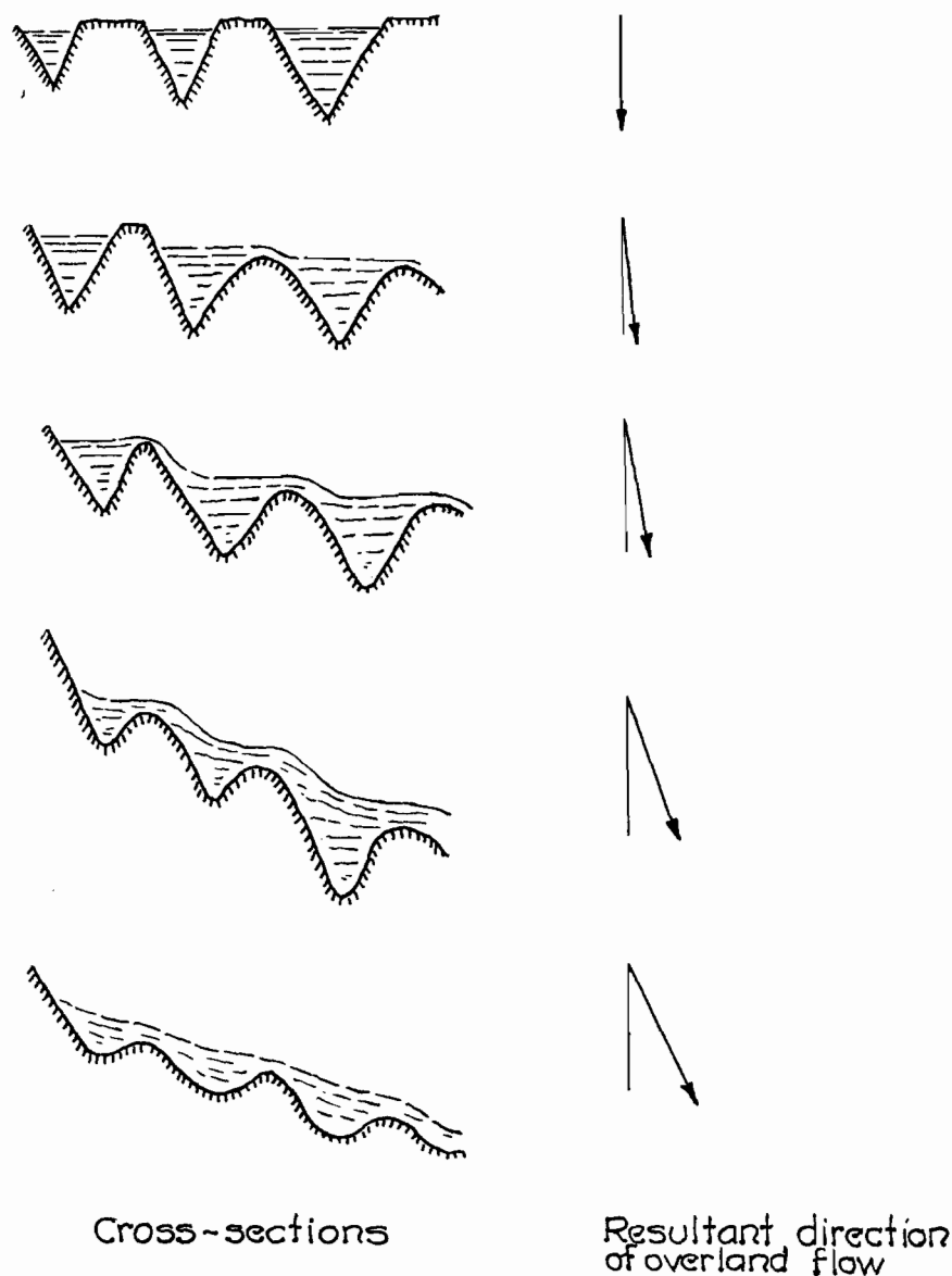
FIGURE 23.— Successive stages of rill obliteration
