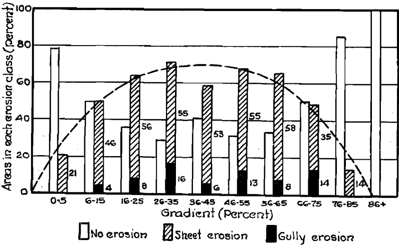
FIGURE 16.—Gradient and degree of erosion (F. G. Renner)
