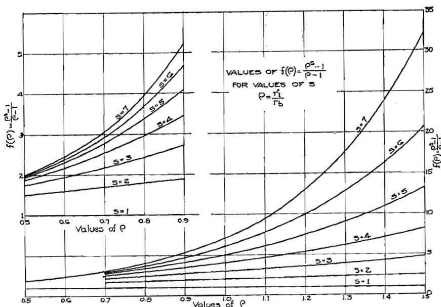
FIGURE 5.—Diagram of factor \rho^s - 1 / \rho - 1
