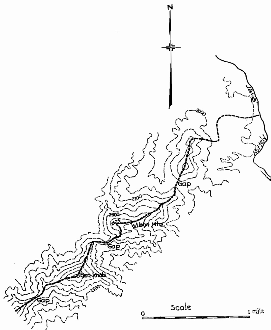
FIGURE 38.— Topography of an interior cross divide (Coosa Bald, Ga., quad., U. S. G. S.—T. V. A.)
