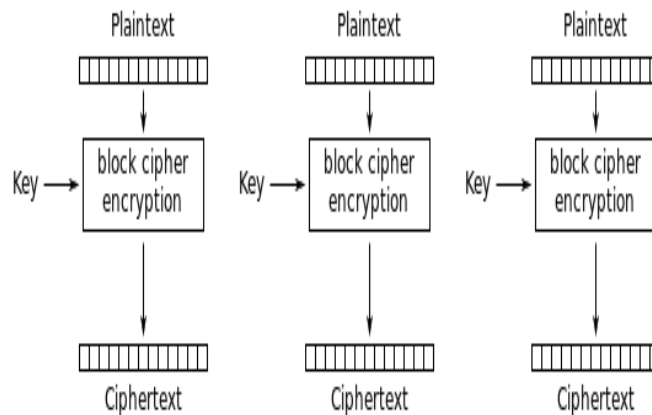
Figure 1. ECB Mode of Operation
