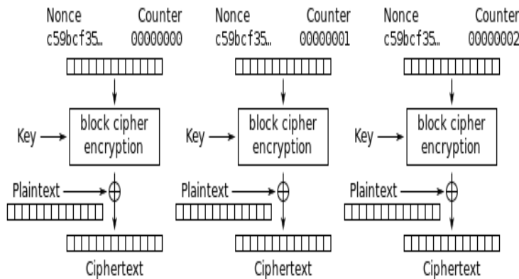
Figure 3. CTR Mode of Operation
