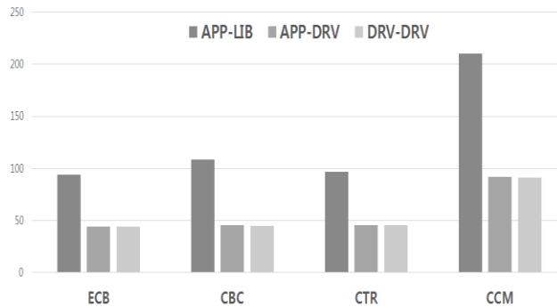
Figure 5. Three Different Interface Calls on ARM9 System
