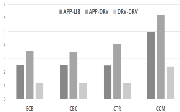
Figure 4. Three Different Interface Calls on x86 System
