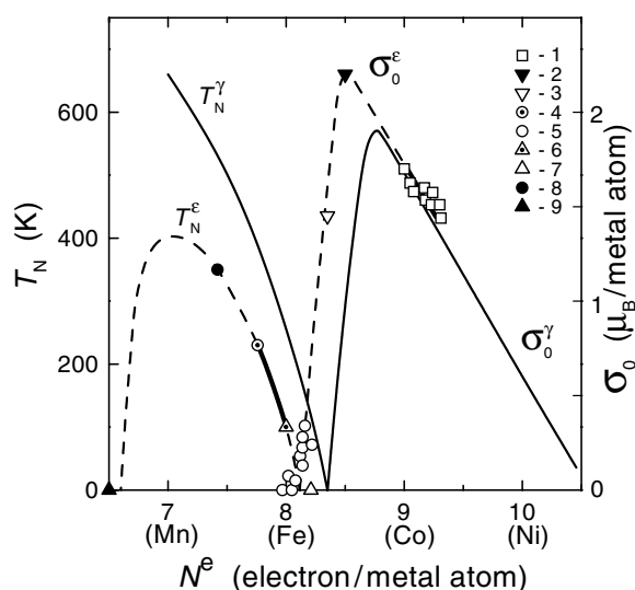
Figure 9. Slater–Pauling curves for fcc ( \gamma ) alloys (experiment—thin solid curves) and hcp ( \epsilon ) alloys (experiment—two sections of thick solid curves; an estimation—dashed curves) of 3d metals that are nearest neighbours in the periodic table. The symbols show experimental data for hydrides presented as a function of the effective electron concentration, N^e(x) = N^e(0) + \eta x , with \eta = 0.5 electrons per H atom: 1— \sigma_0 of \epsilon -CoH _x solid solutions [30]; 2— \sigma_0 of \epsilon' -FeH [19]; 3— \sigma_0 of Fe _{0.947} Cr _{0.053} H _{0.92} with a 9R-type metal lattice [16]; 4— T_N of \epsilon -Fe [31]; 5— \sigma_0 of \epsilon -FeH _{0.42} [18]; 6— T_N of \epsilon -Fe _{0.776} Mn _{0.224} [32]; 7— \sigma_0 of \epsilon -Fe _{0.776} Mn _{0.224} H _x solid solutions [33]; 8— T_N of \epsilon -Mn _{0.83} [34]; 9— T_N of \epsilon -CrH [35].
