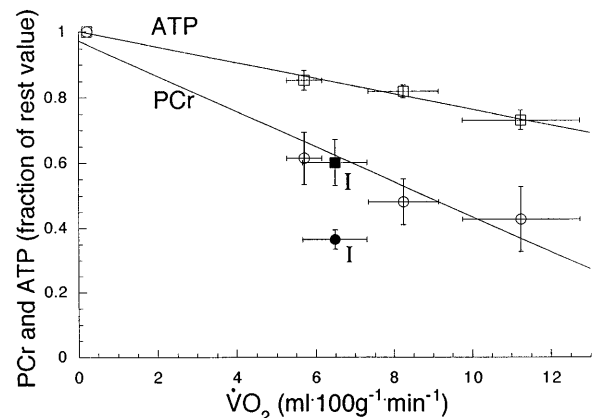
Fig. 5. Relationship between PCr ( \bullet , \circ ; n = 4 ) and ATP ( \blacksquare , \square ; n = 5 ; as fraction of rest values) and \dot{V}O_2 for the 3 contraction periods at which blood flow was normal ( \square , \circ ) and I contraction period ( \blacksquare , \bullet ). Values are means \pm SE. Correlation lines are only drawn from regression analysis (best fit) by using the 3 stimulation patterns with unrestricted blood flow.
