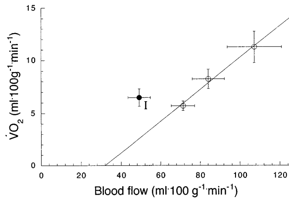
Fig. 2. Relationship between muscle \dot{V}O_2 and muscle blood flow for the 3 contraction periods at which blood flow was normal ( \circ ) and I contraction period ( \bullet ). Values are means \pm SE. Correlation line is drawn from regression analysis (best fit) by using the 3 stimulation patterns with unrestricted blood flow.
