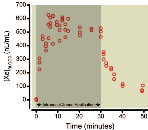
Fig. 3. Blood gas analysis. Concentrations of xenon measured in the blood ( [Xe]_{\text{BLOOD}} ) of the internal jugular vein of two volunteers. Intranasal application of xenon for 30 min at a rate of 1.0 l/h followed by 20 min of washout using oxygen at a rate of 8 l/min. A steady state was reached within approximately 10 min providing evidence for a direct pathway from nose to brain.
