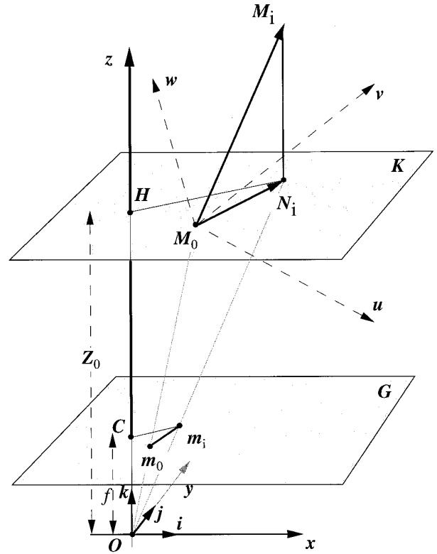
FIG. 2. The initial loop in POSIT looks for a pose of the object such that the points m_i are the scaled orthographic projections of the object points M_i .
