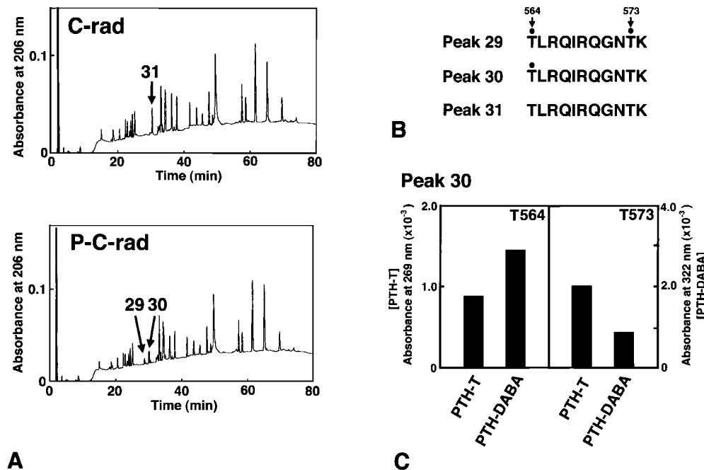
Figure 2. Determination of amino acid residues of radixin that are phosphorylated by Rho-kinase. (A) Comparison of elution profiles of lysyl endopeptidase-digested peptides of non- and fully phosphorylated C-rad from reverse-phase HPLC (C-rad and P-C-rad, respectively). Rho-kinase-dependent phosphorylation divided and shifted the peak 31 from nonphosphorylated C-rad into two peaks, peaks 30 and 29, from phosphorylated C-rad. For details see the text. (B) Amino acid sequences of peaks 29, 30, and 31. The PTH-threonine/PTH-dehydroaminobutyric acid ratio (see C) revealed that T564/T573 in peak 29 and T564 in peak 30 were phosphorylated (Kato et al., 1994; Fujita et al., 1996). (C) The PTH-threonine/PTH-
