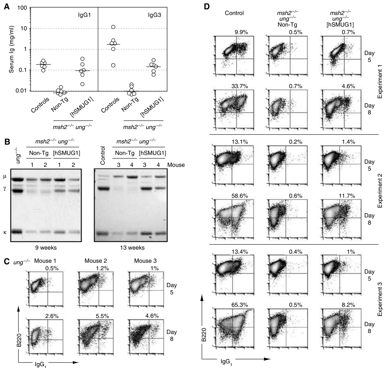
Figure 2 SMUG1 overexpression in msh2^{-/-}ung^{-/-} mice allows the accumulation of substantial levels of serum IgG. (A) Titres of IgG1 and IgG3 in sera of mice of different genotypes (aged 9–20 weeks) as determined by ELISA. The mice analysed were the products of crosses between msh2^{+/-}ung^{-/-} [hSMUG1] transgenic males and msh2^{+/-}ung^{-/-} non-transgenic females, with age-matched C57BL/6 mice providing controls. (B) Serum immunoglobulin profiles of four msh2^{-/-}ung^{-/-} control and four msh2^{-/-}ung^{-/-} [hSMUG1] transgenic mice analysed at the ages indicated. Representative examples of sera from age-matched normal and ung^{-/-} mice are shown for comparison. Total serum immunoglobulin was precipitated using protein L-agarose, resolved by SDS-PAGE and stained with Coomassie blue. (C) Flow cytometric profiles of three independent experiments in which splenic B cells from UNG-deficient mice were cultured in the presence of LPS + IL4 for 5 or 8 days prior to staining for slgG1 and CD45R(B220). Live cells were gated by staining with propidium iodide, and percentages of slgG1 + B cells are indicated. (D) Flow cytometric profiles of three independent experiments in which splenic B cells from msh2^{-/-}ung^{-/-} [hSMUG1]-transgenic, msh2^{-/-}ung^{-/-} control or wild-type mice were cultured in the presence of LPS + IL4 for 5 or 8 days prior to staining for slgG1 and CD45R(B220). Live cells were gated and percentages indicated as in panel C.
