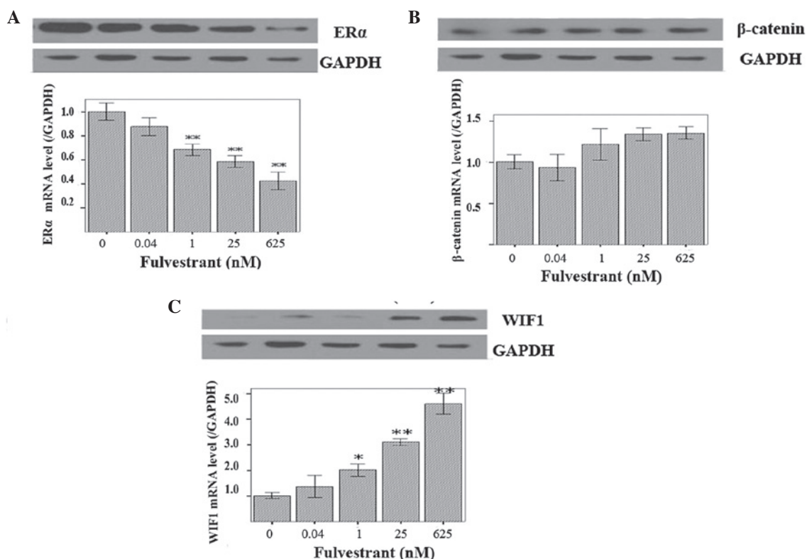
Figure 3. Protein and mRNA expression of (A) ER \alpha , (B) \beta -catenin and (C) WIF1 in the HepG2 cell line treated with different concentrations (0.04, 1, 25 and 625 nM) of fulvestrant. The columns show the mean of three samples per group; the bars show the standard deviation. *P<0.05 and **P<0.01 vs. 0 nM group. ER \alpha , estrogen receptor \alpha ; WIF1, Wnt inhibitory factor-1.
