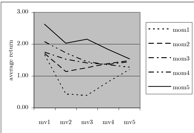
Figure 11: Interaction: size-momentum
