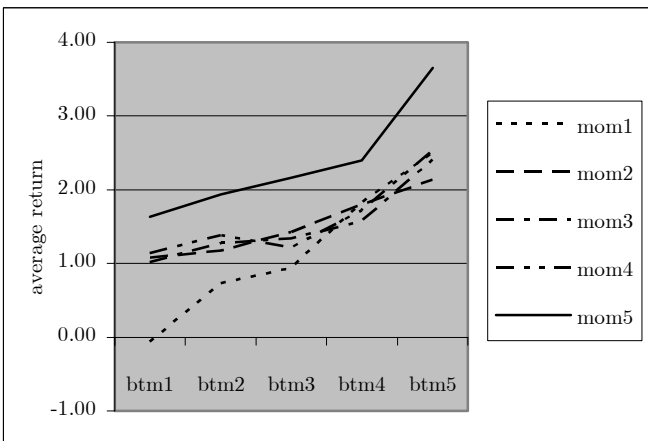
Figure 12: Interaction: distress-momentum
