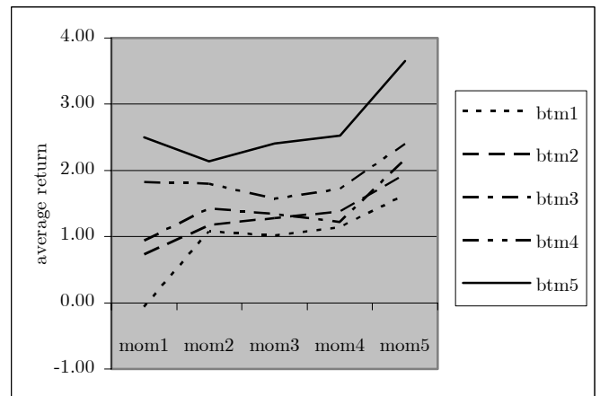
Figure 15: Interaction: distress-momentum
