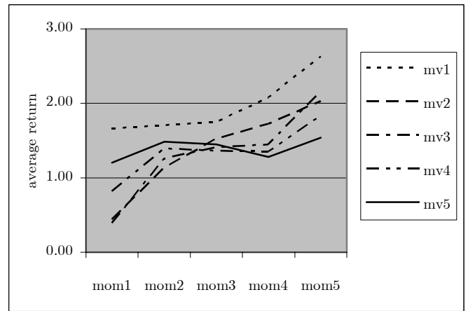
Figure 14: Interaction: size-momentum
