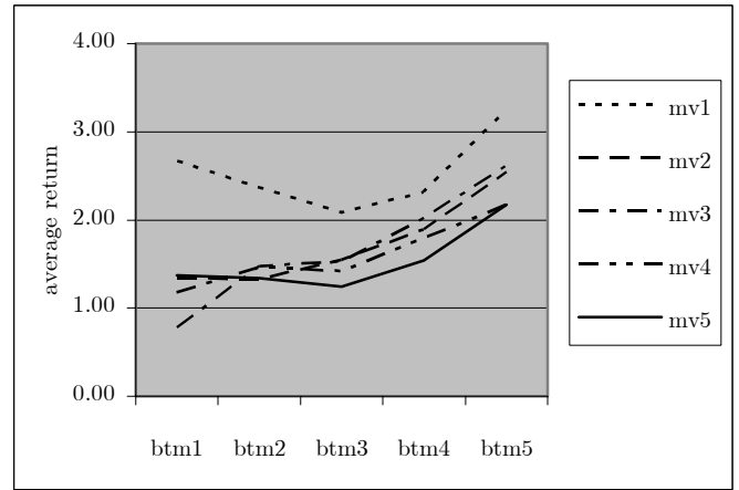
Figure 13: Interaction: size-distress
