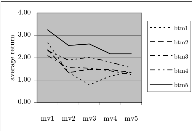
Figure 10: Interaction: size-distress
