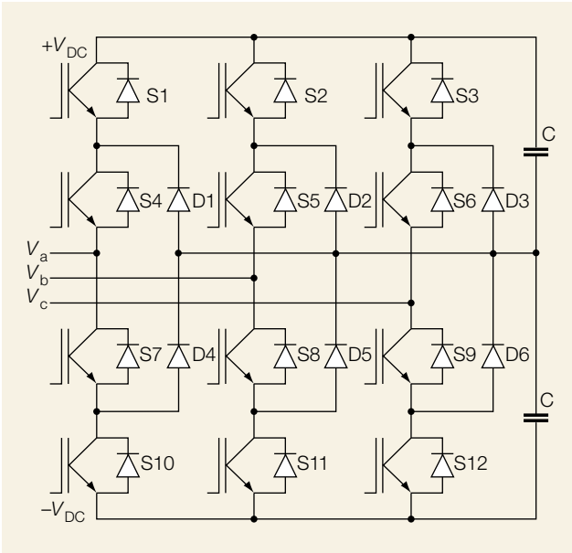
Basic three-level voltage source converter
