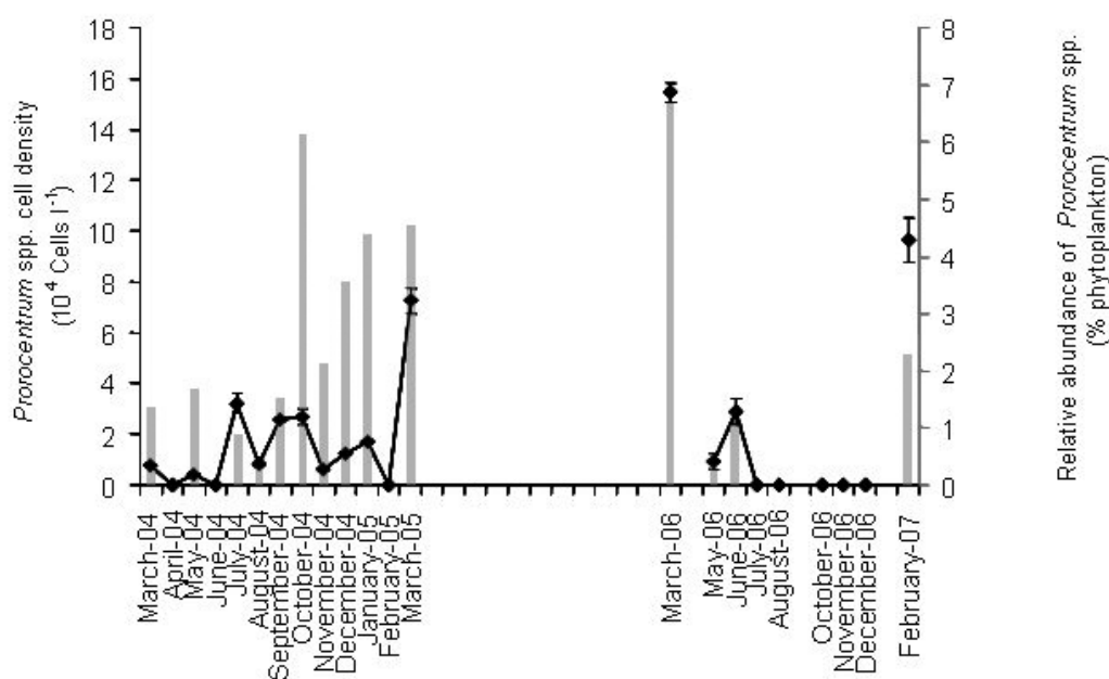
Fig. 3: Monthly variation in total (Line and scatter plot, Mean ± SD, n=3) and relative abundance (grey bars) of Prorocentrum spp. at the sampling station, Bizerte Lagoon (March 2004 - March 2005/ March 2006 - February 2007).
