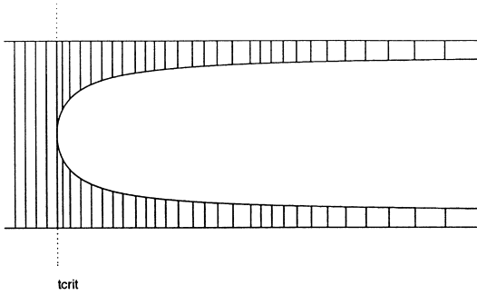
FIG. 2. Plot of the support J as a function of t , for the case V = tx^2 , t > 0 .
