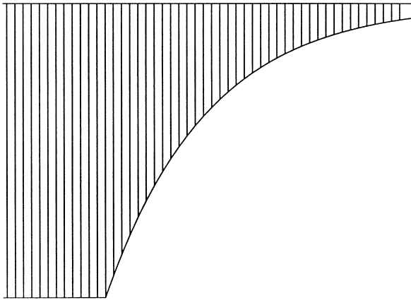
FIG. 5. Plot the support J as a function of t , for the case V = tx , t > 0 .
