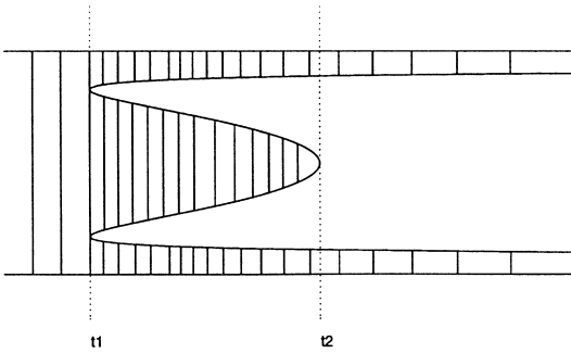
FIG. 3. Plot of the support J as a function of t , for the case V = tx^4 , t > 0 .
