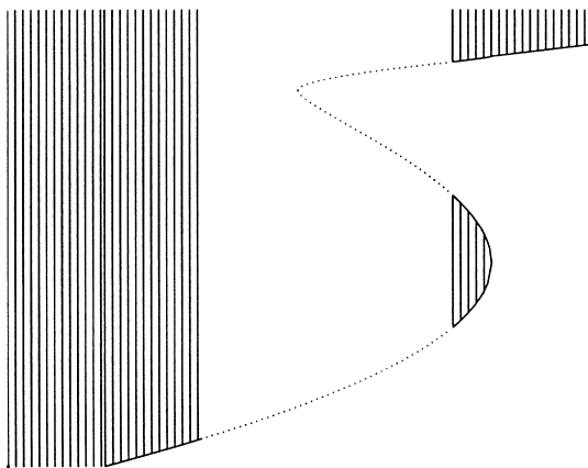
FIG. 7. Plot of the support J as a function of t , for the general case V = tX^{2q+1} , t > 0 , q \geq 2 . The dotted lines denote our conjecture for the region t_{+, 2q+1} + \epsilon < t < t_{+, 2q+1}^{(1)} - \epsilon .
