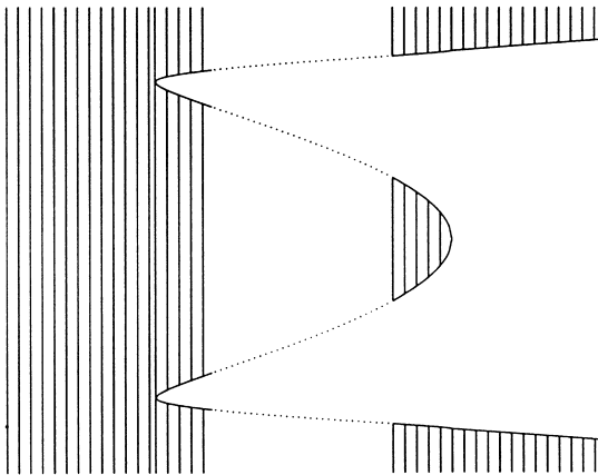
FIG. 4. Plot of the support J as a function of t , for the general case V = tx^{2q} , t > 0 , q \geq 3 . The dotted lines denote our conjecture for the region t_{+, 2q} + \varepsilon < t < t_{+, 2q}^{(1)} - \varepsilon .
