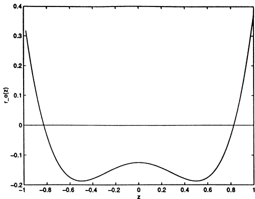
FIG. 8. Plot of r_0(z) for q=2 . Note two minima (in plot, at locations \pm\beta^* = \pm\frac{1}{2} ).
