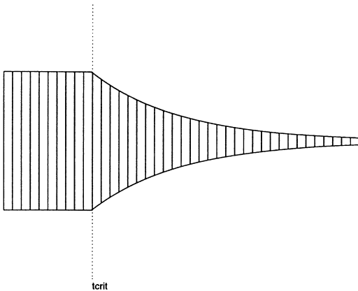
FIG. 1. Plot of the support J as a function of t , for the case V = -tx^{2q} , t > 0 .
