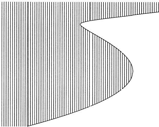
FIG. 6. Plot of the support J as a function of t , for the case V = tx^3 , t > 0 .
