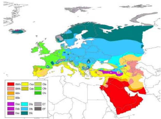
Fig. 8. Köppen-Geiger climate type map of Europe.
