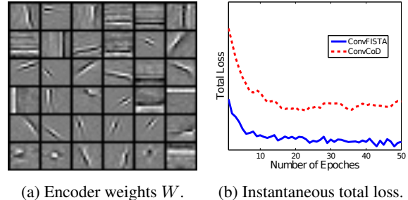
Fig. 3: (a) Shows 36, 11 \times 11 encoder filter weights learned using ConvFISTA. They resemble in the learned dictionary filters (not shown). (b) Shows the instantaneous total loss at every epoch for both ConvFISTA and ConvCoD.
