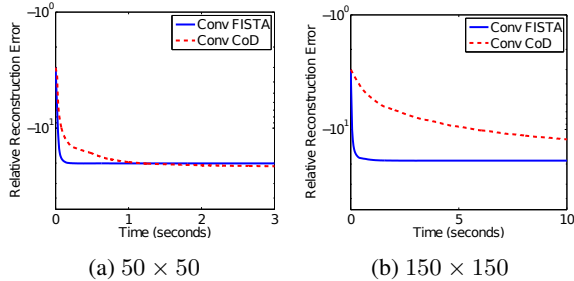
Fig. 2: Comparison of the convergence rate between convolutional CoD (ConvCoD) and convolutional FISTA (ConvFISTA). Two different images sizes, (a) 50 \times 50 pixel and (b) 150 \times 150 pixel, are used for comparison.
