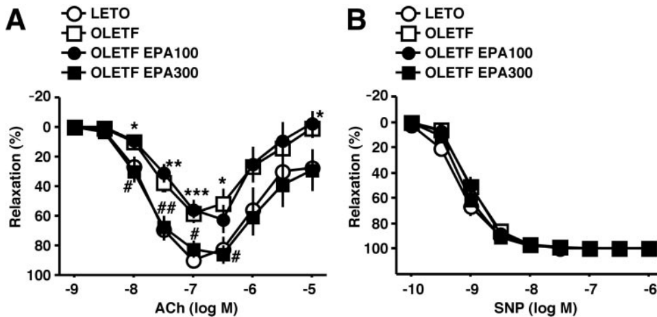
Fig. 1. EPA improves endothelium-dependent relaxation in OLETF rats. Concentration-response curves for ACh (A)- and SNP (B)-induced responses in isolated rings of mesenteric arteries obtained from LETO, OLETF, and EPA (100 or 300 mg/kg/day for 4 weeks)-treated OLETF (EPA100 or EPA300) rats. Details are given under Materials and Methods . Data are means \pm S.E.M. from n = 8 (A) or n = 5 (B) experiments. *, P < 0.05; **, P < 0.01; and ***, P < 0.001, LETO versus OLETF group. #, P < 0.05; and ##, P < 0.01, OLETF versus EPA300 group.
